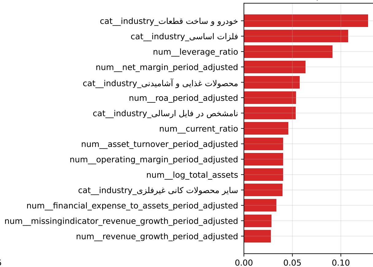
XGBoost importance
