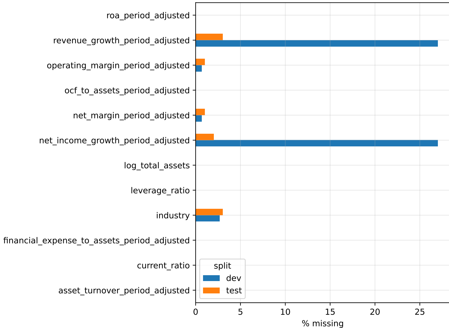
Missingness by split
