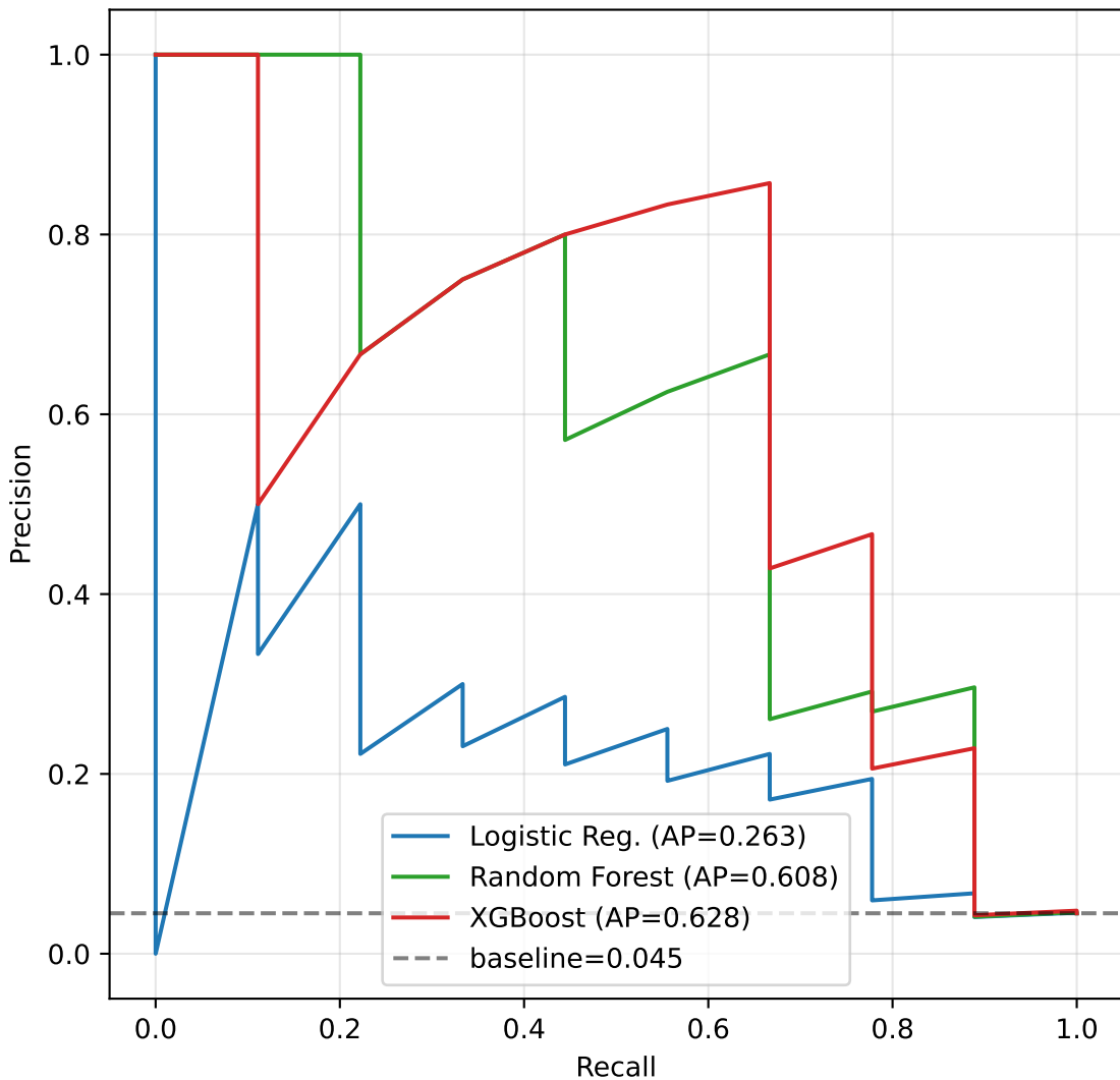
Precision-Recall — test
