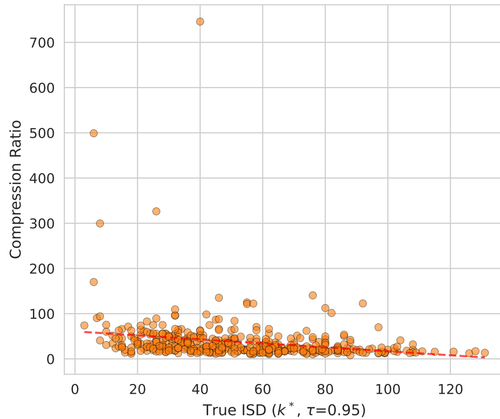
(B) ISD vs Compression r=-0.218 , N=419
