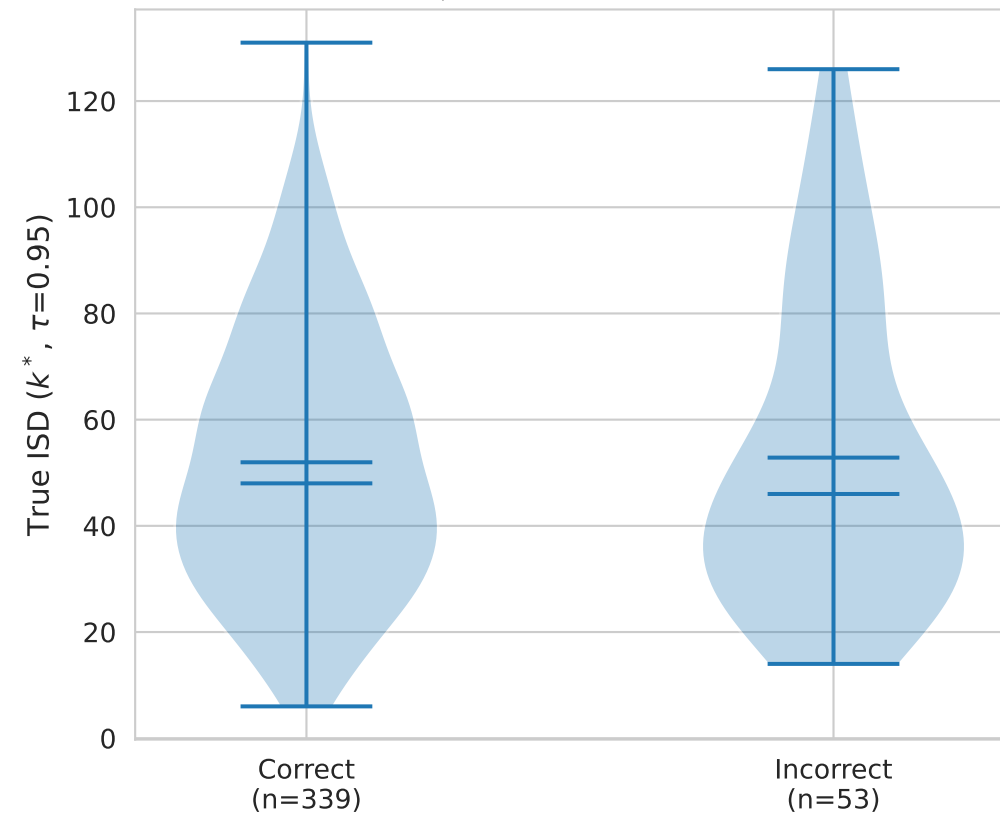
(C) ISD by Topic Accuracy r_{pb}=-0.012 , N=392
