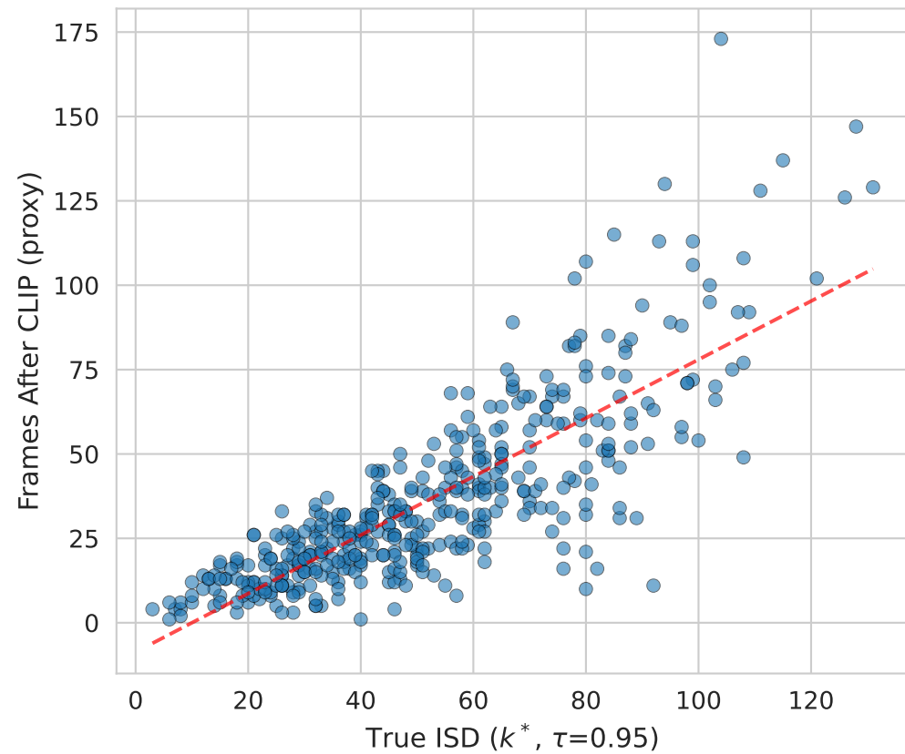
(A) ISD vs Proxy r=0.816 , \rho=0.819 , N=419
