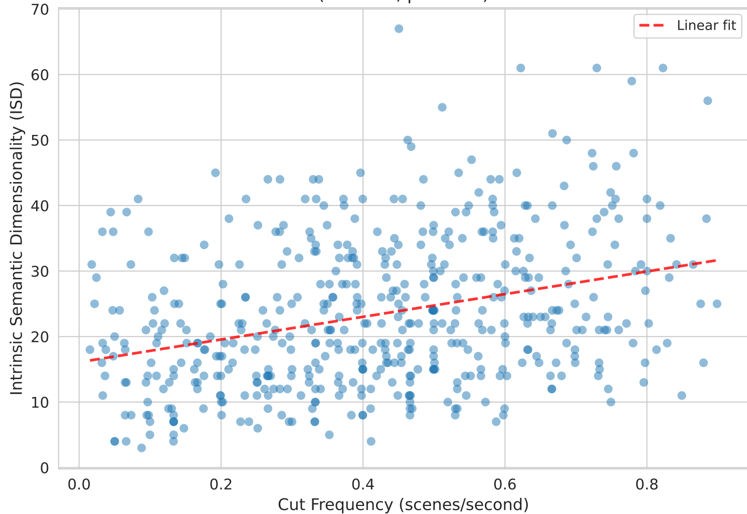
ISD Captures Editing Complexity ( r=0.322 , p<0.001 )
