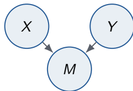
Collider
