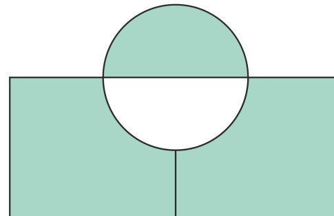
Symmetric difference
