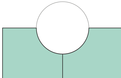
Difference
