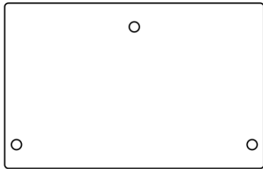
MULTIPOINT
