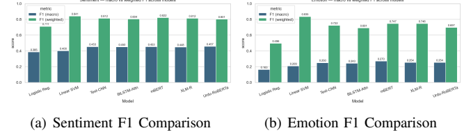
Fig. 7. Gaps between Macro-F1 and Weighted-F1 across sentiment and emotion tasks, showing majority-class bias.
