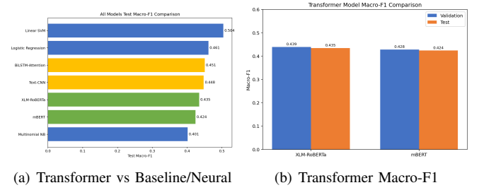
Fig. 6. Fine-tuned Transformer models compared to deep sequence and traditional classifiers.
