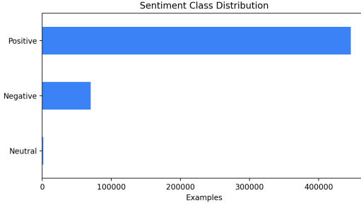
Fig. 4. Preprocessed class frequency distribution highlighting massive imbalance.
