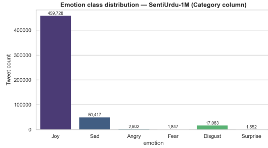
Fig. 3. Canonical emotion distribution in the labeled local corpus before empty-cleaned-text removal.
