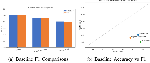
Fig. 5. Baseline model metrics highlighting the tradeoff between overall accuracy and minority class F1 scores.
