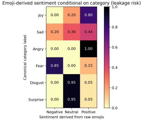
Fig. 2. Conditional association between sentiment derived from raw emojis and canonical categories. Strong cells indicate a shortcut risk if emojis remain in the input.
