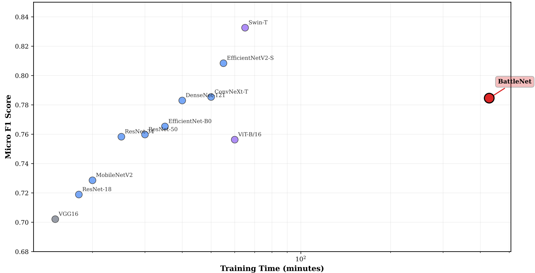
Model Efficiency: F1 vs Training Time
