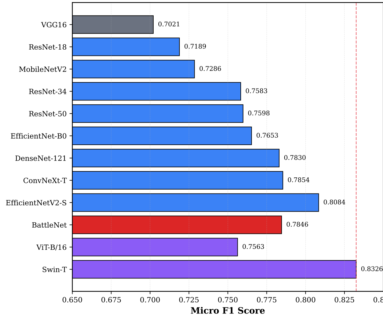
(a) Micro F1 Score by Architecture
