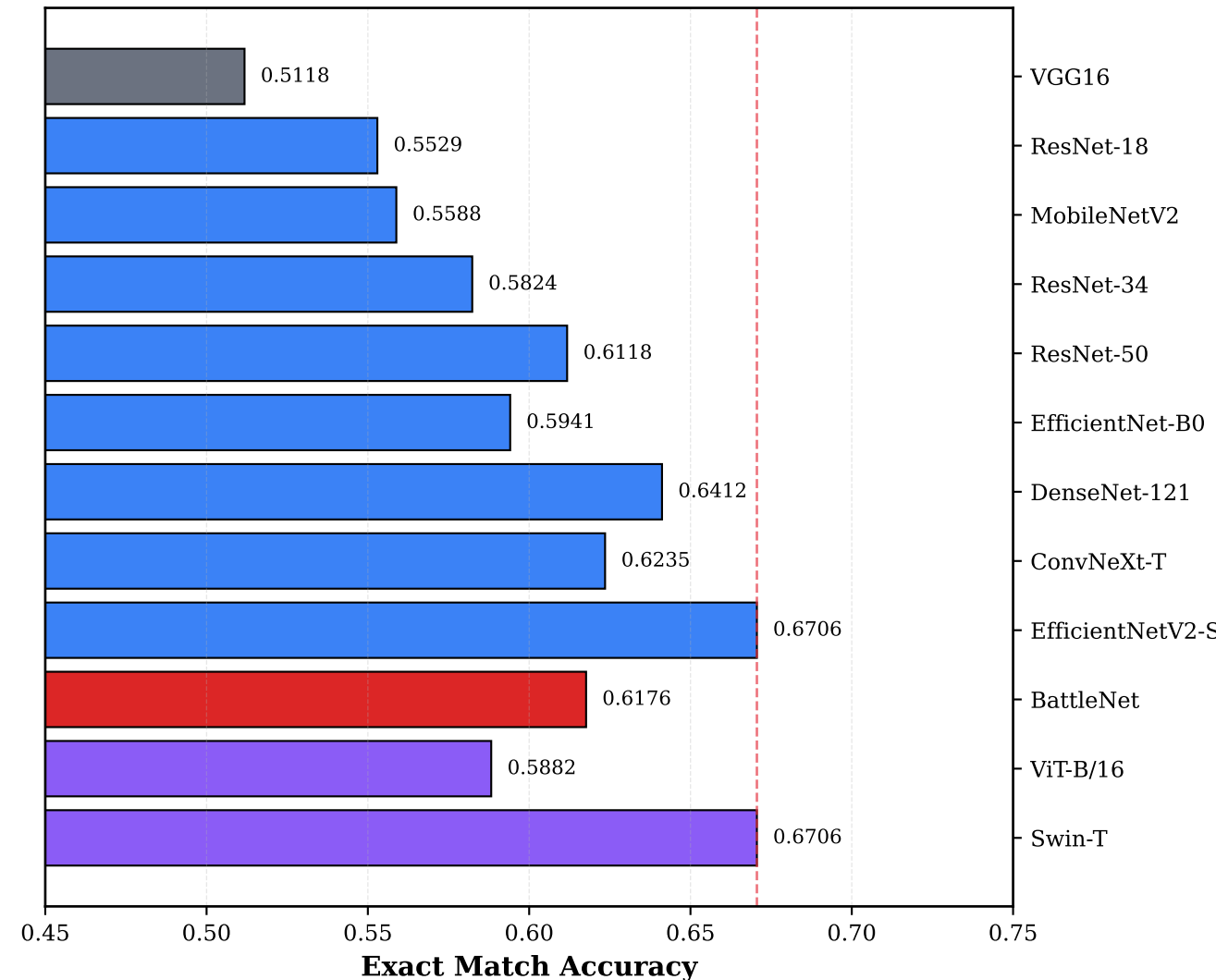
(b) Exact Match Accuracy by Architecture
