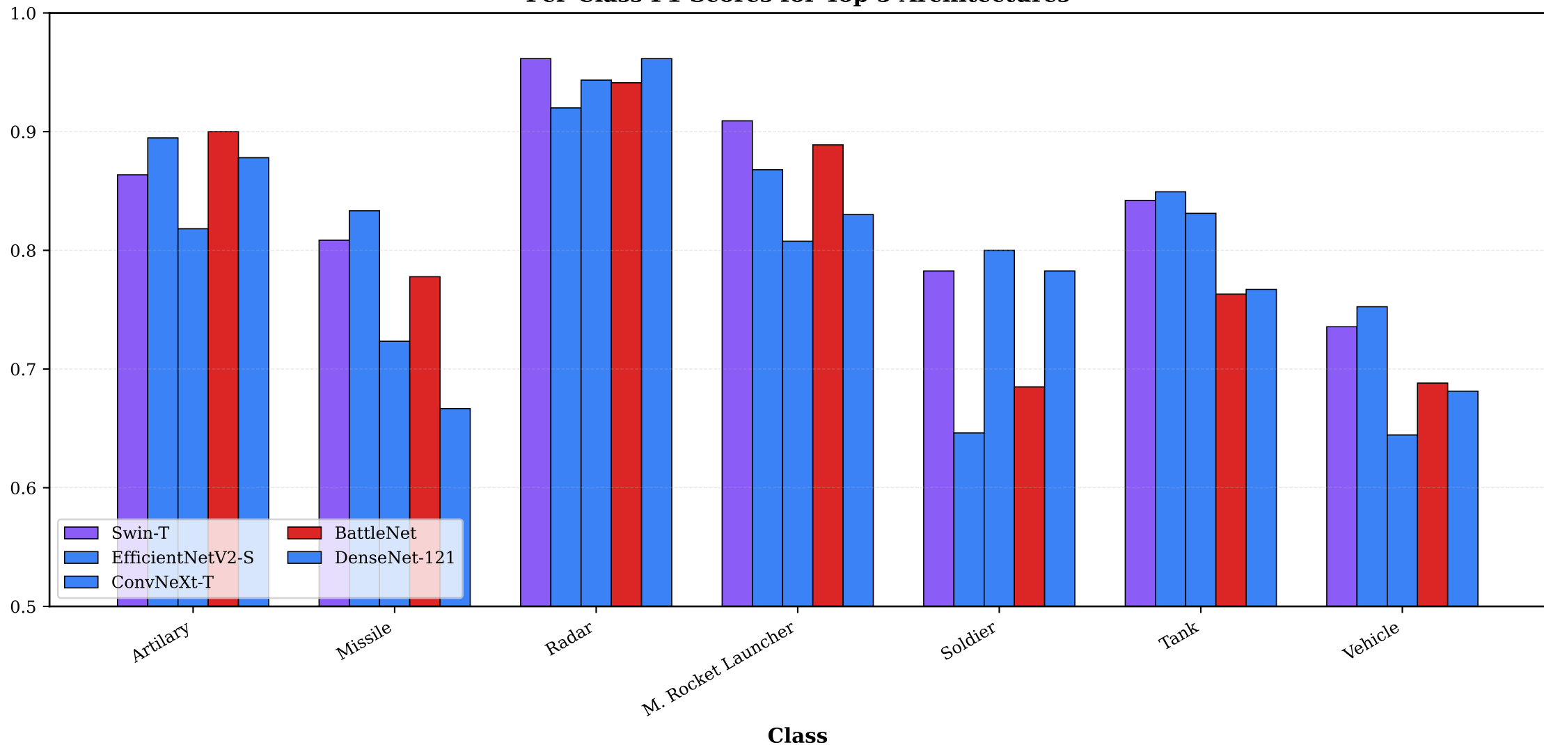
Per-Class F1 Scores for Top 5 Architectures
