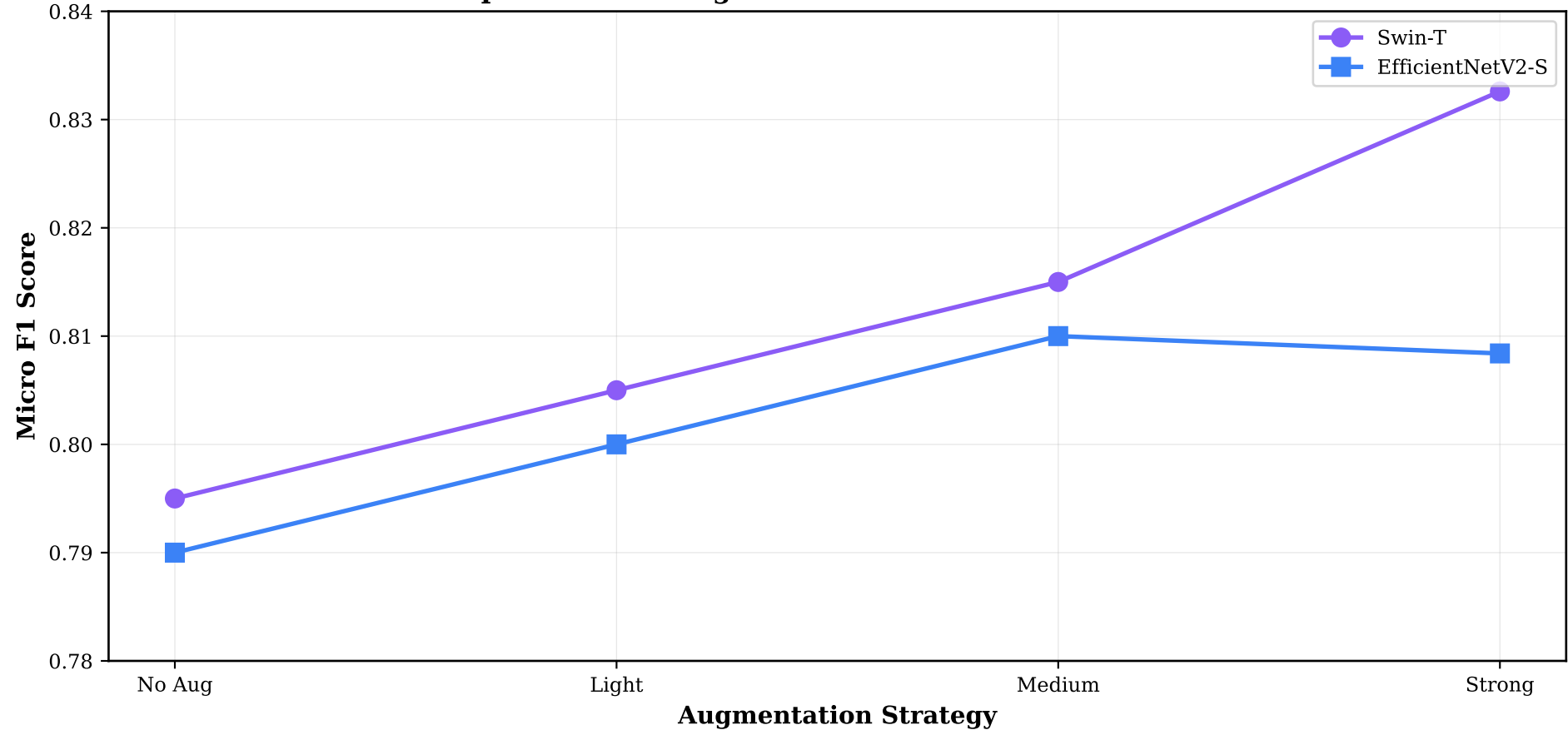
Impact of Data Augmentation on Model Performance
