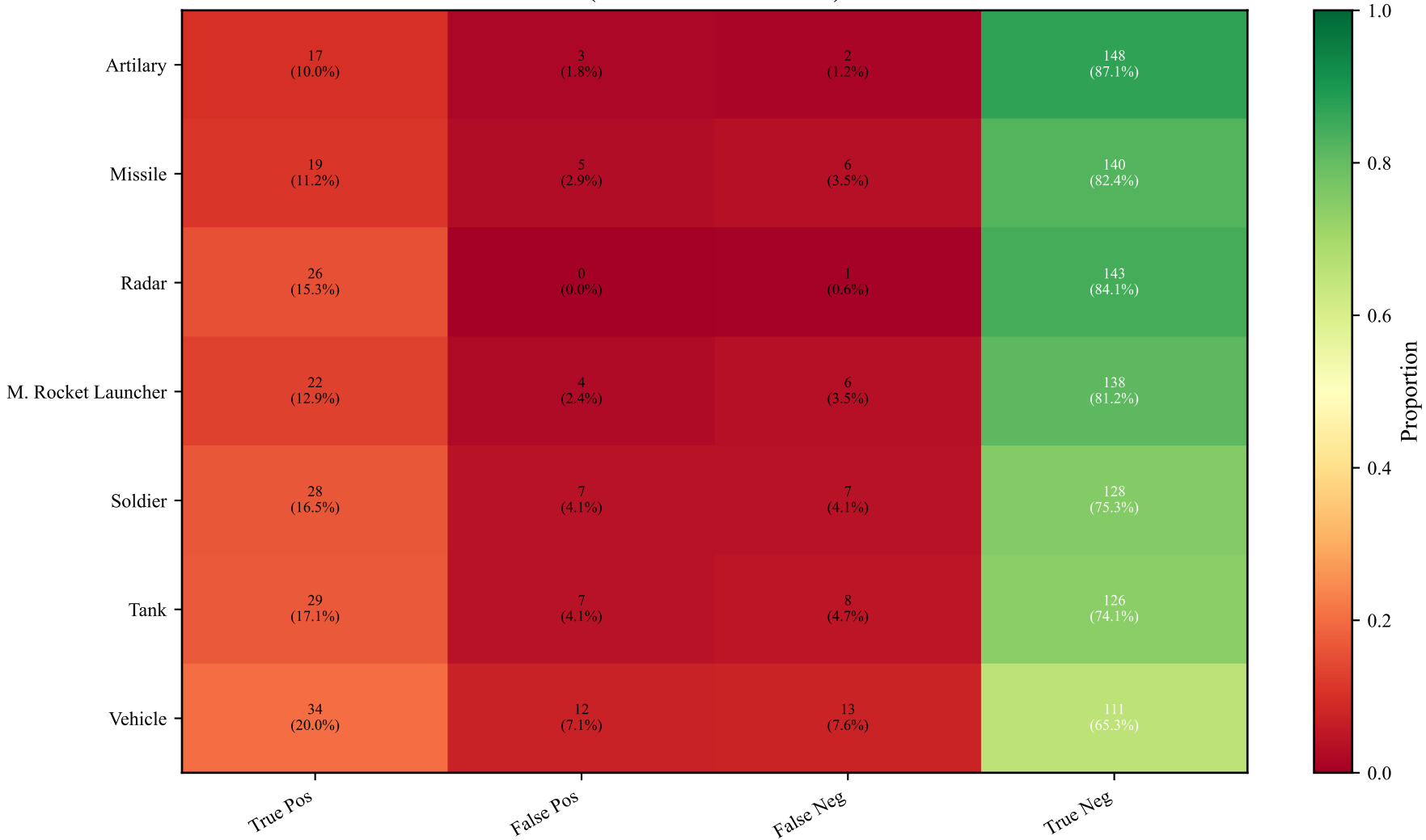
Per-Class Confusion Analysis — Swin-T Baseline (Values: Count / Row %)
