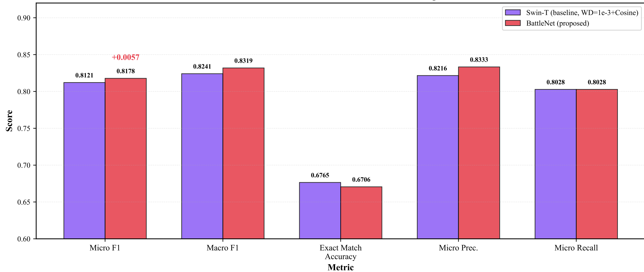
BattleNet vs. Swin-T Baseline: All Metrics Comparison
