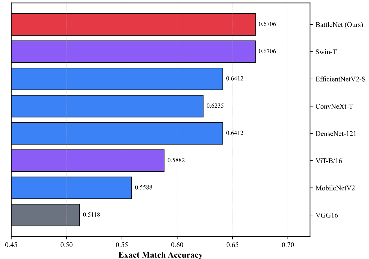
(b) Exact Match Accuracy by Architecture
