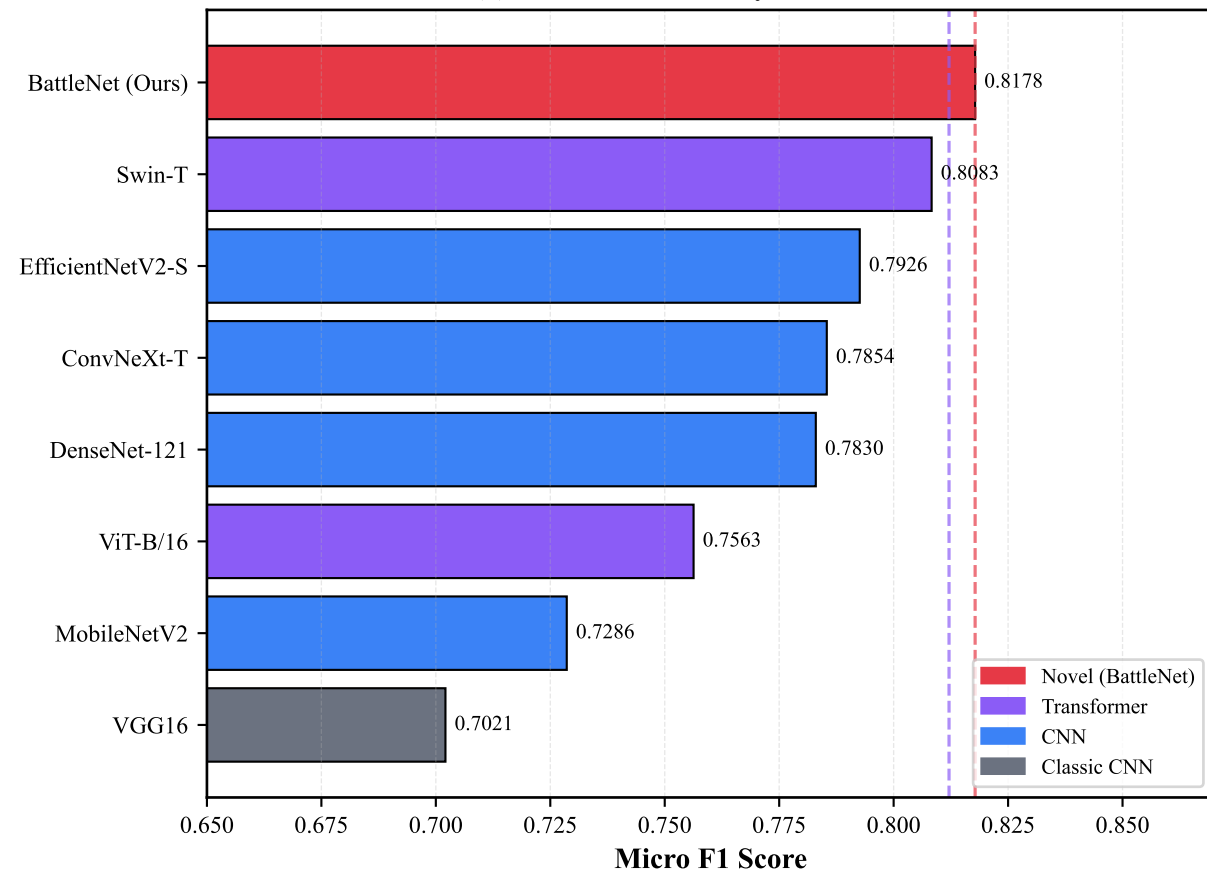
(a) Micro F1 Score by Architecture
