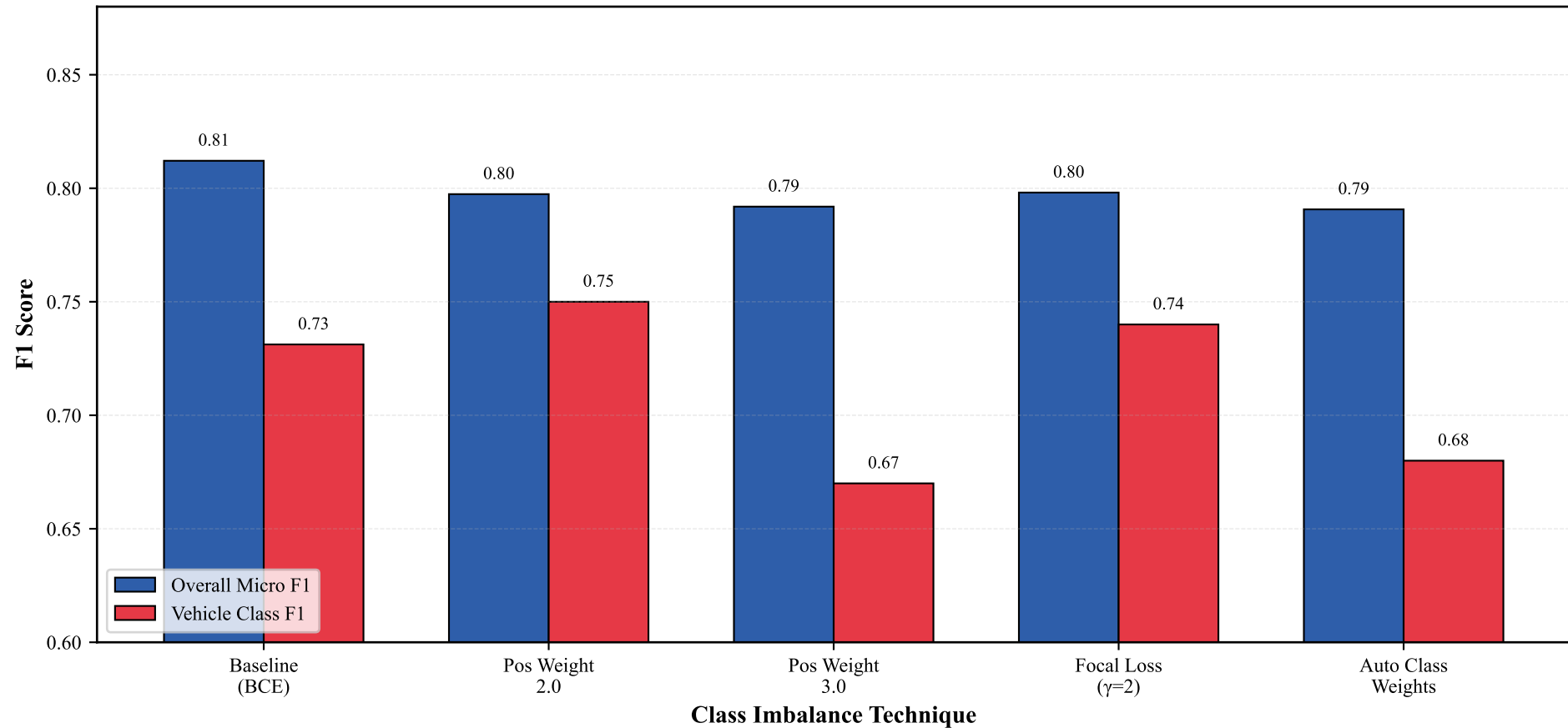
Impact of Class Imbalance Techniques on Swin-T (WD=1e-3 + Cosine)
