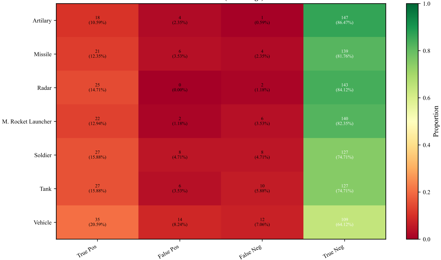
Per-Class Confusion Analysis for Swin-T (Best Model) Values: Count (Percentage)
