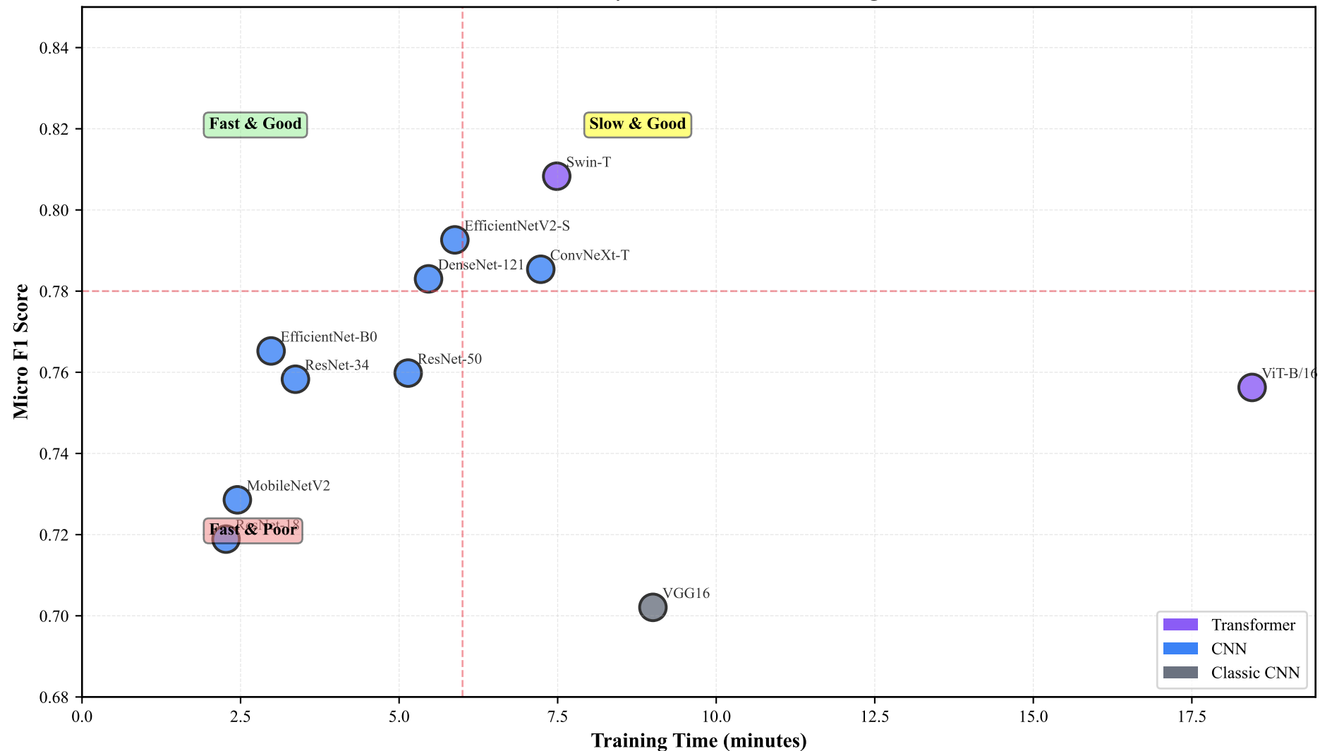
Model Efficiency: Performance vs Training Time
