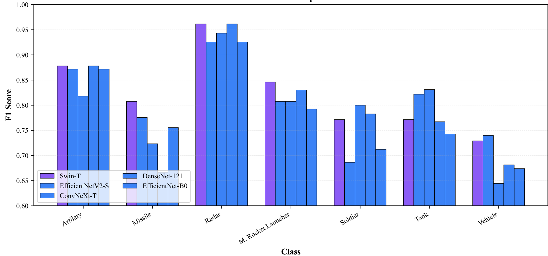
Per-Class F1 Scores for Top 5 Architectures
