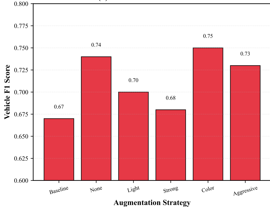
(b) Vehicle Class Performance
