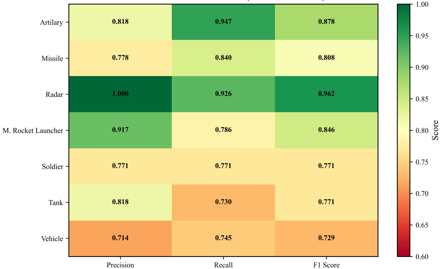
Per-Class Metrics for Swin-T (Best Architecture)
