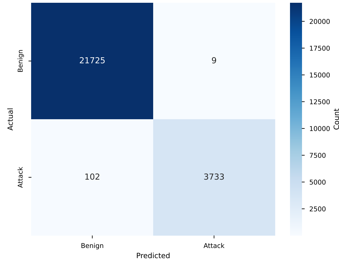
(c) LightGBM F1=98.54%
