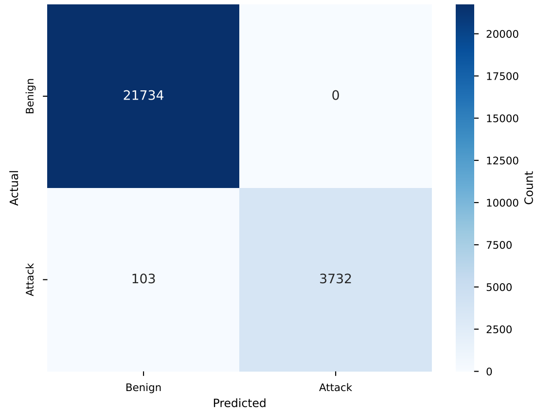
(a) Voting Ensemble F1=98.64%
