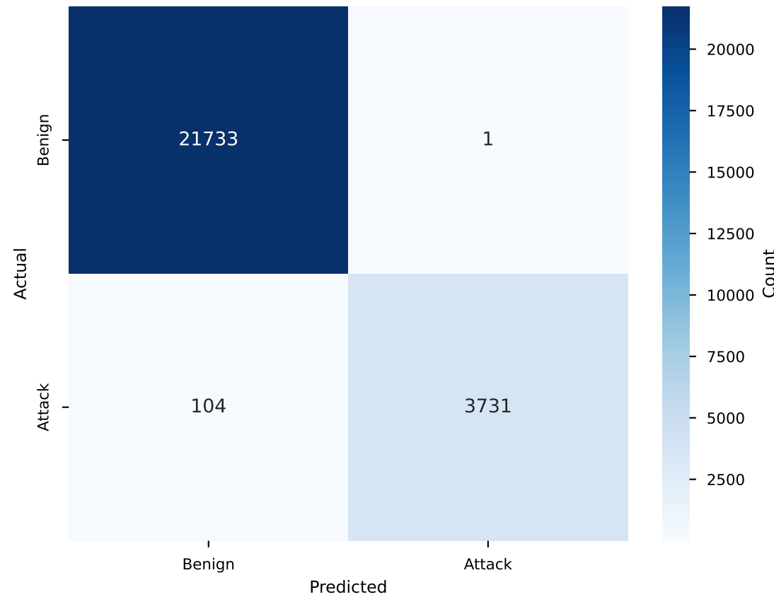
(b) XGBoost F1=98.61%
