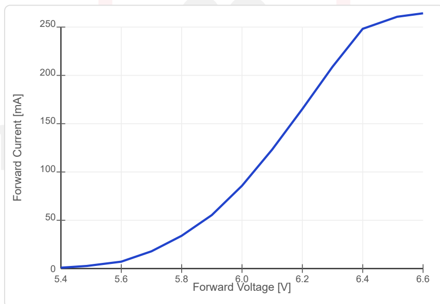
Figure4: Chip Forward Current Characteristics
