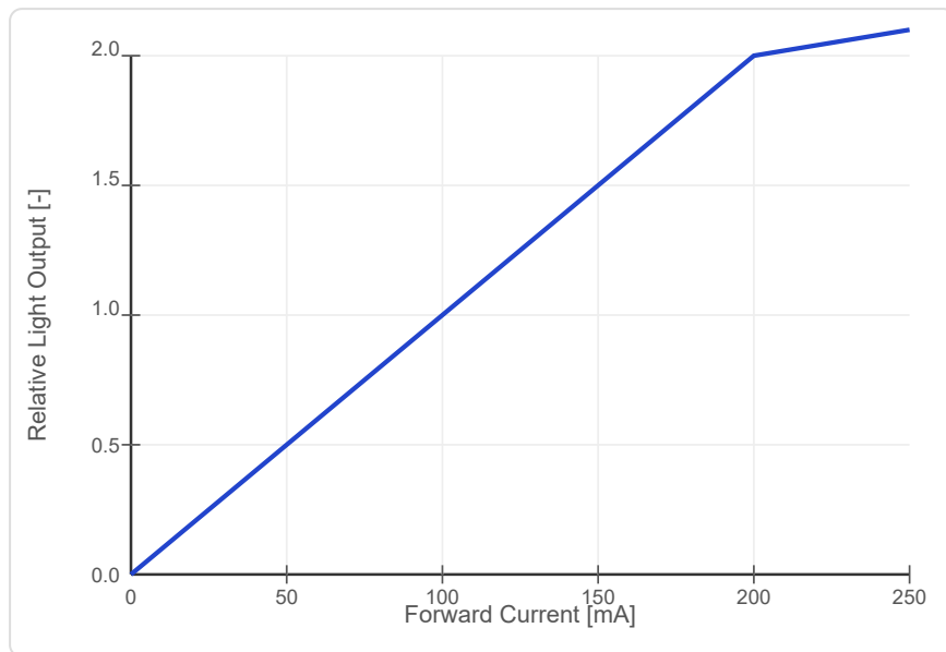
Figure3.b: Chip Light Output Characteristics
