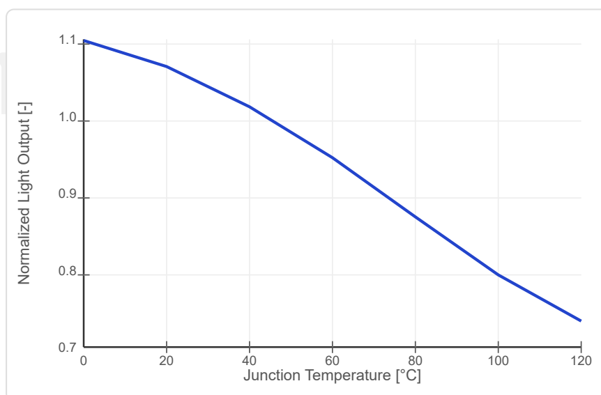
Figure3.a: Chip Light Output Characteristics
