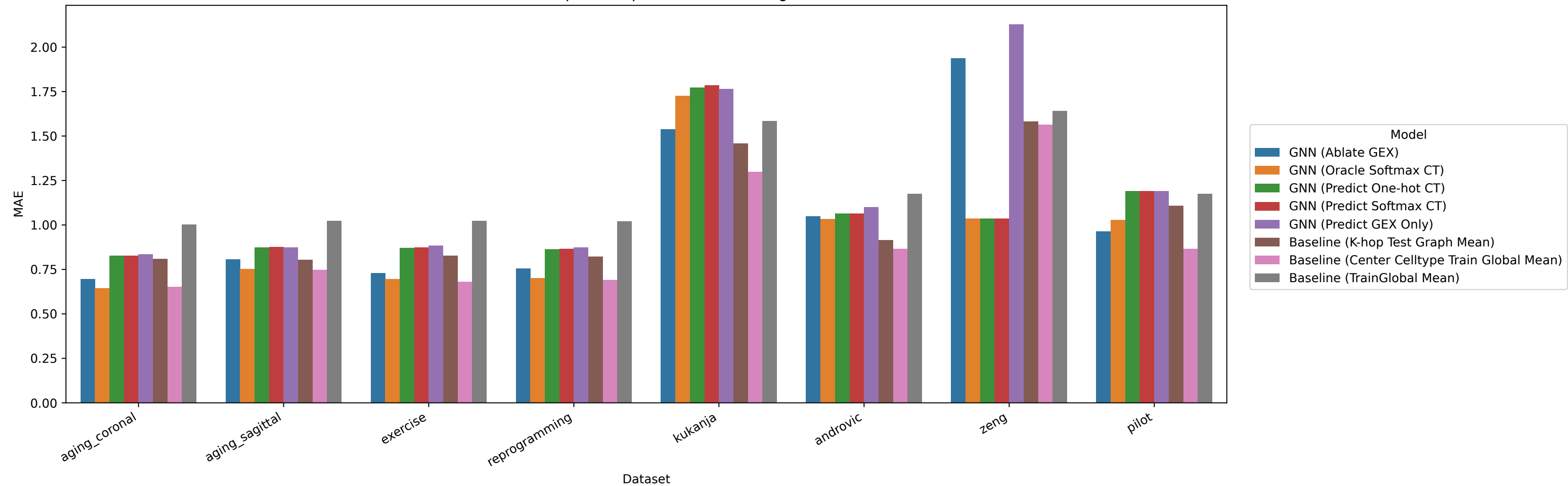
Center cell expression prediction (MAE, all genes)
