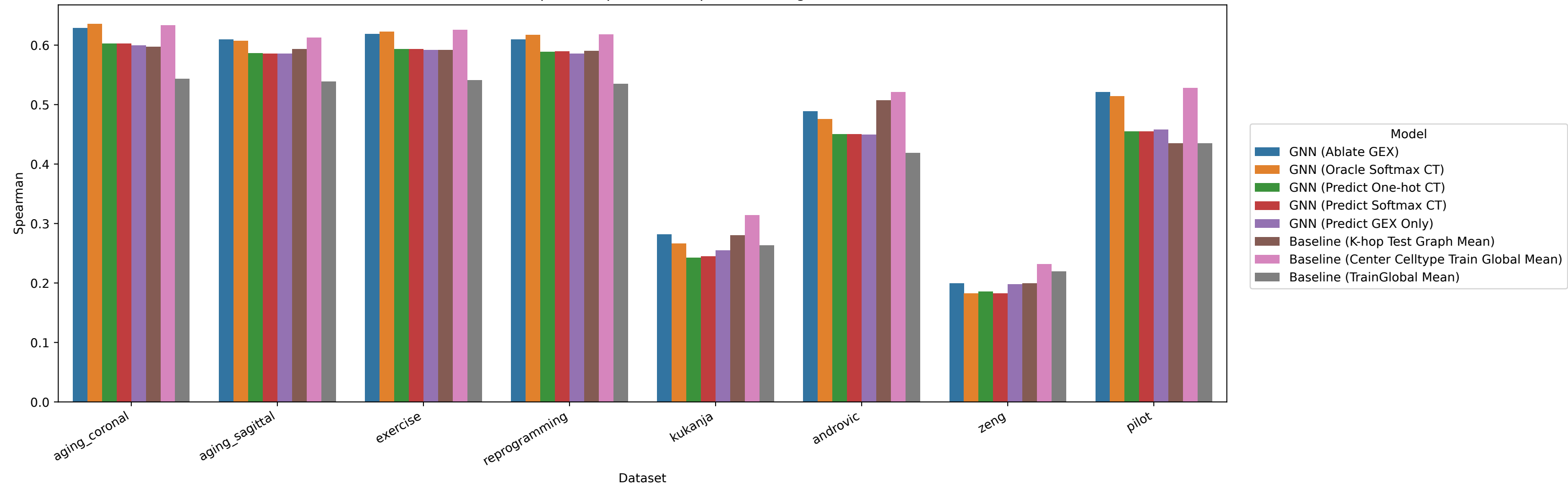
Center cell expression prediction (Spearman, all genes)
