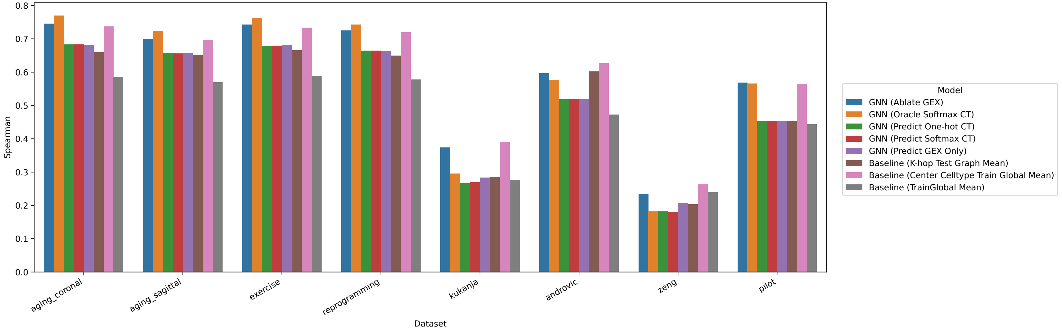
Center cell expression prediction (Spearman, nonzero genes)
