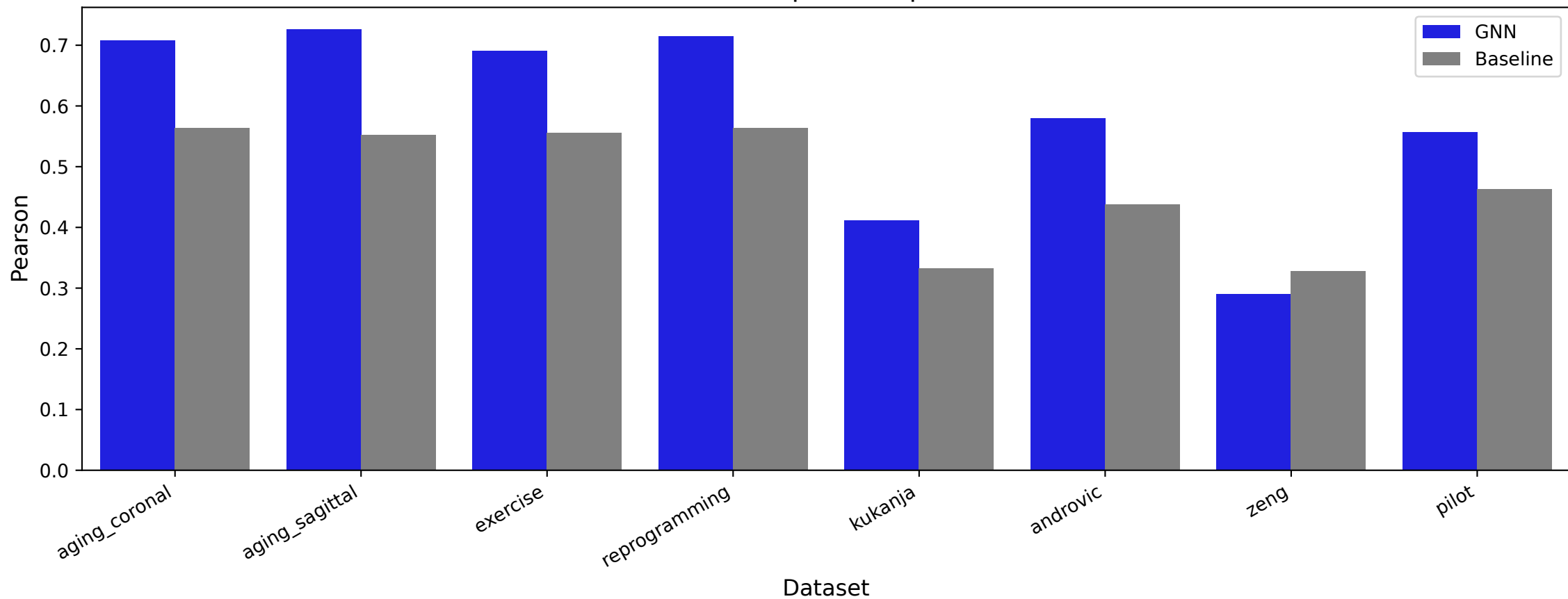
Center cell expression prediction
