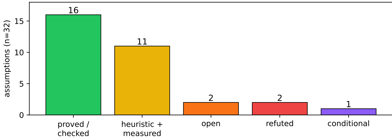
IC-for-ECDLP assumption graph: status summary (from DOT source)
