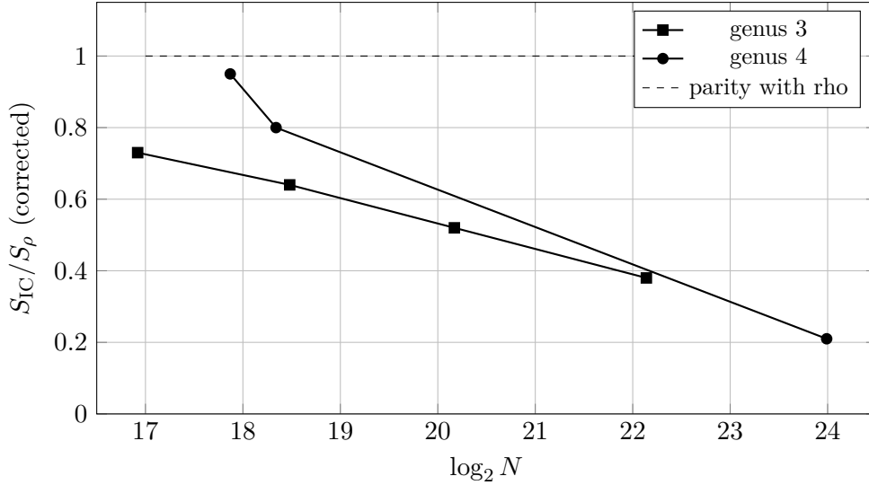
Figure 2: Hyperelliptic positive control. The ratio to distinguished-point rho falls at genus 3 and genus 4 with the predicted slopes. No measured end-to-end elliptic variant of Sections 9.2 and 9.3 has crossed this line.
