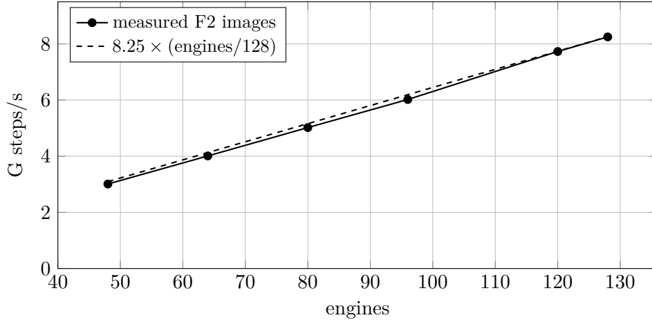
Figure 1: Companion ECC2K-130 FPGA engine on AWS F2. The 128-engine image at 333 MHz is 8.25 G steps/s. Linear scaling with engine count is the prediction of a design that shares nothing between engines except the host port. This library’s digit-serial core is not on this figure: it has no fmax.
