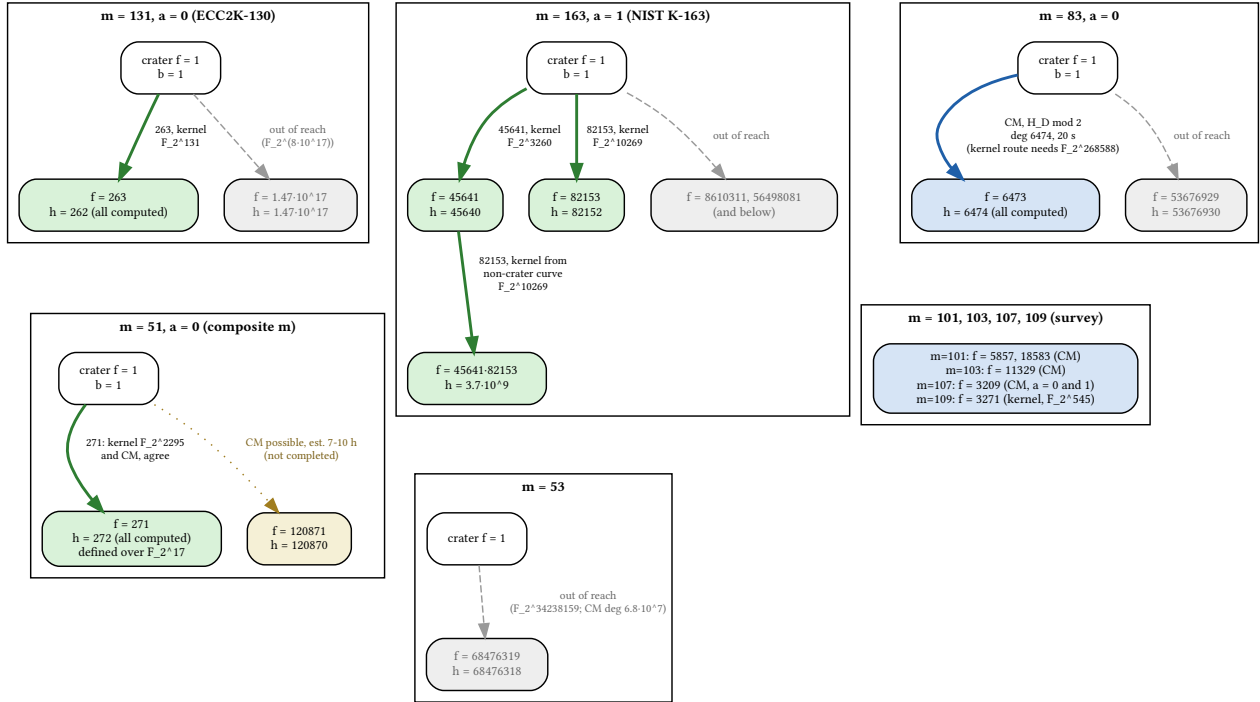
Figure 2: Conductor levels reached on each Koblitz class, and the route used. Green: kernel route (Vélu on kernel points). Blue: CM route. Dotted: estimated, not completed. Grey dashed: out of reach. Source: reachability.dot.
