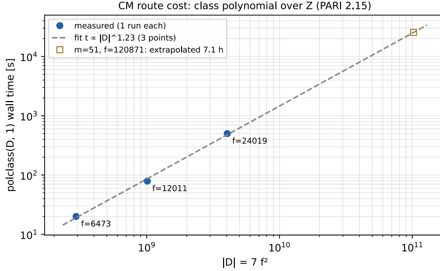
Figure 3: \text{polclass}(D, 1) wall time against |D| ; one run per point; dashed: power-law fit; square: extrapolation to the m = 51 120871-floor. Source: cm_route/scale_polclass.out , cm_route/plot_scaling.py .
