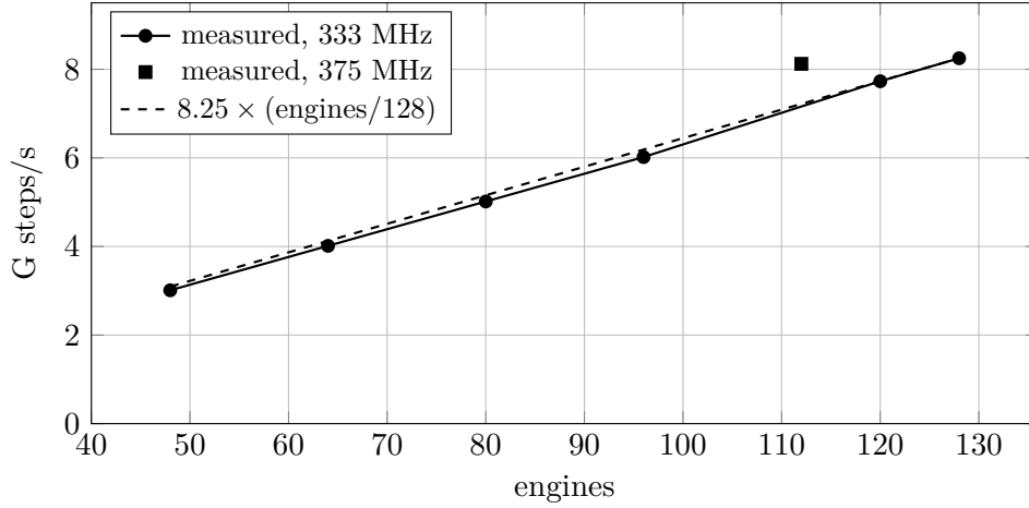
Figure 1: ECC2K-130 FPGA engine on AWS F2. The 128-engine image at 333 MHz is 8.25 G steps/s; the pre-board estimate was 5–12 G with a central 8 G. The measurement landed on the central estimate and is a device number, not the estimate reprised.
