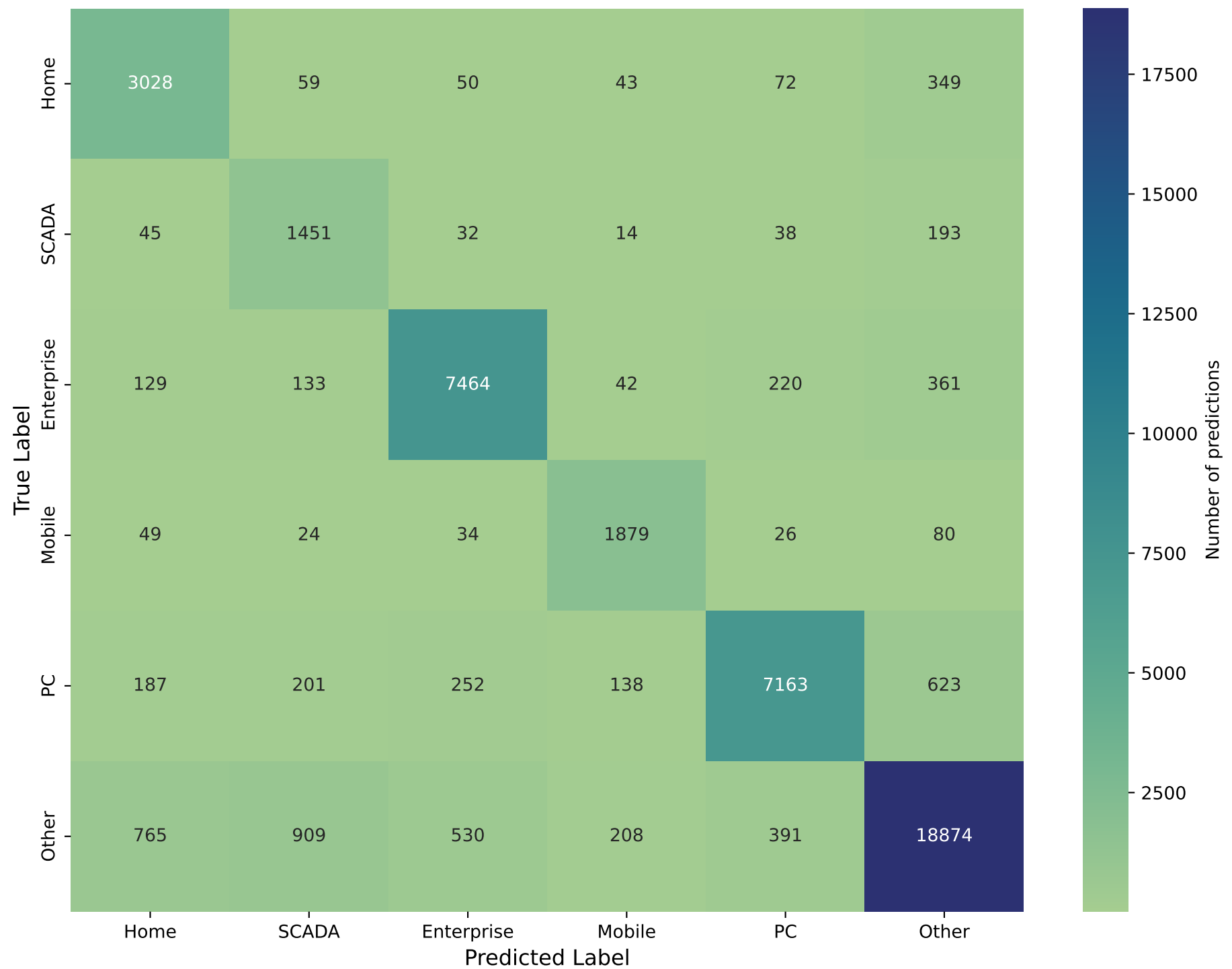
Confusion Matrix - Balanced Linear SVM
