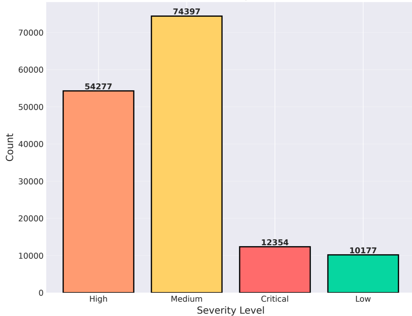
CVSS Severity Counts
