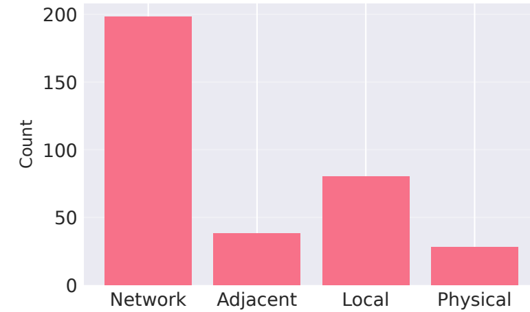
Attack Vector
