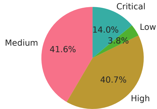
Severity Distribution
