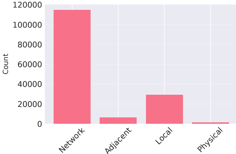
Attack Vector
