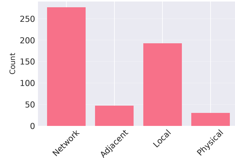
Attack Vector
