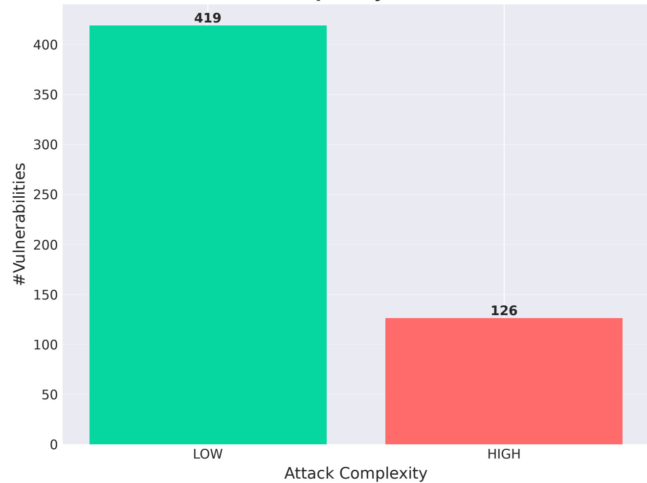
Attack Complexity Distribution
