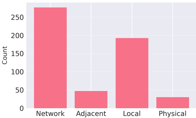
Attack Vector
