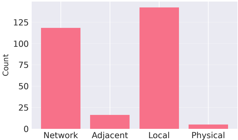
Attack Vector
