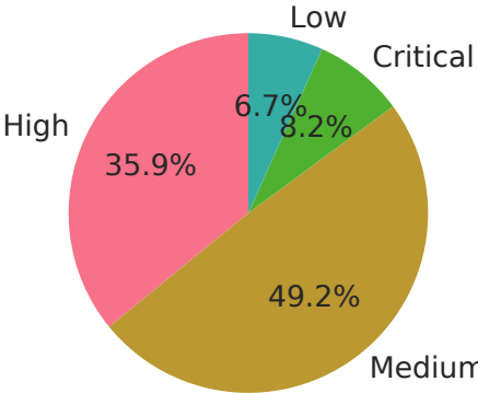
Severity Distribution
