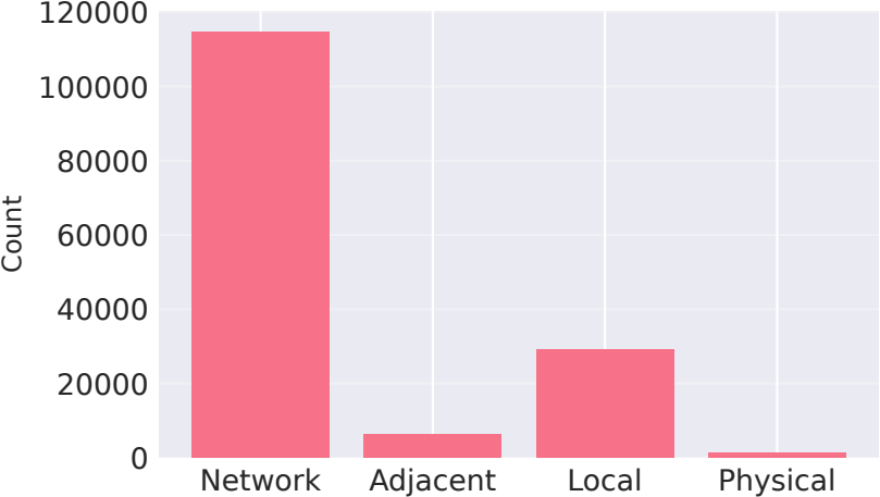
Attack Vector
