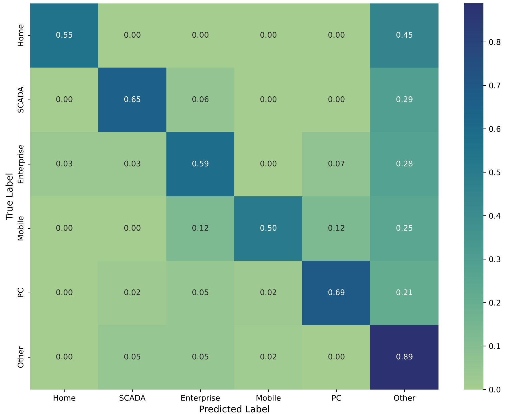
Normalized Confusion Matrix - Balanced Linear SVM
