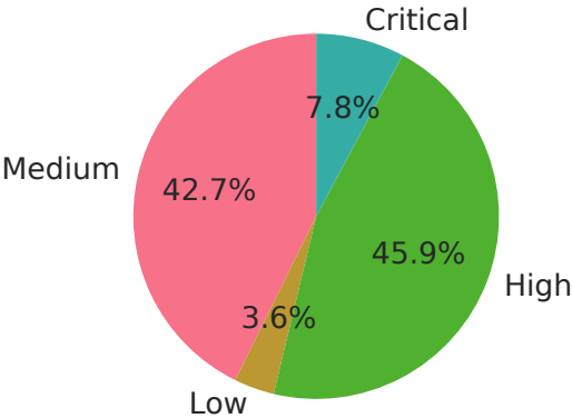
Severity Distribution
