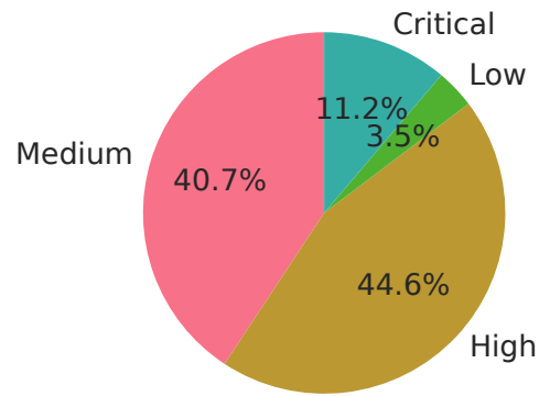
Severity Distribution
