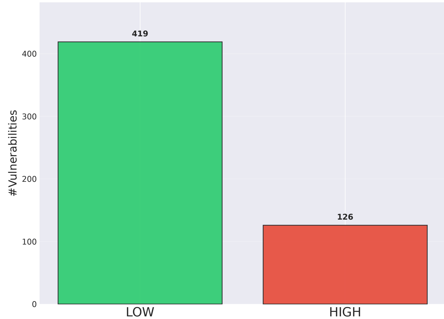
Attack Complexity
