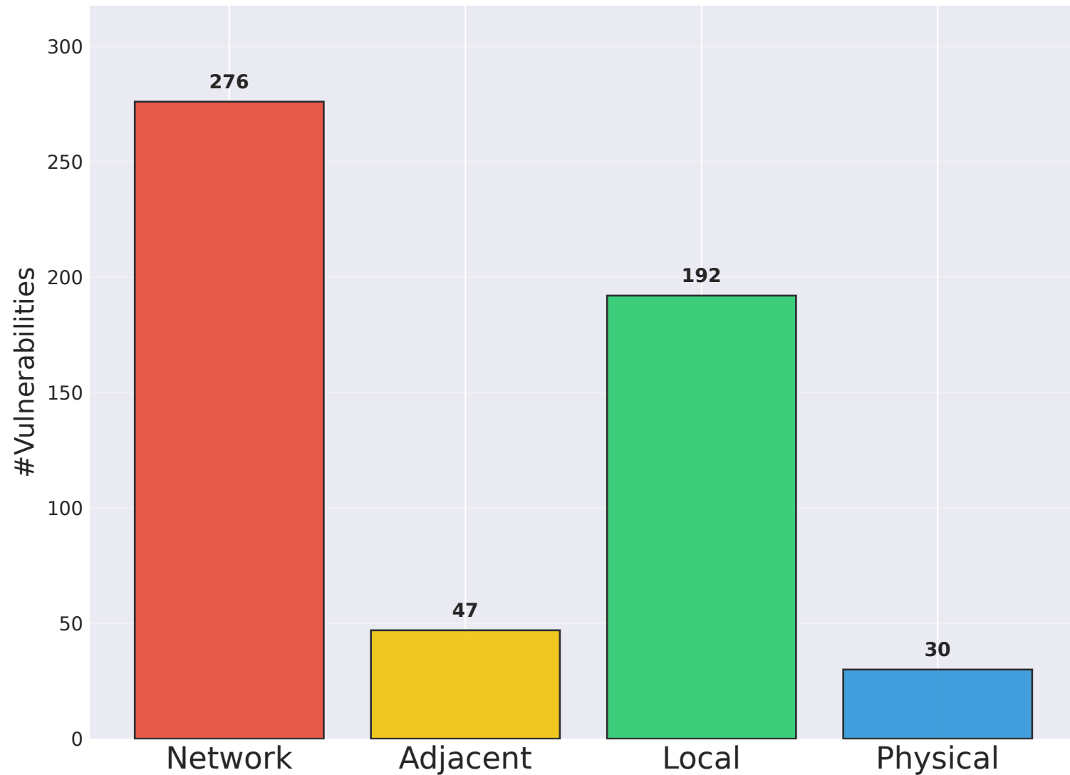
Attack Vector
