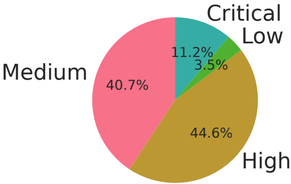
Severity Distribution
