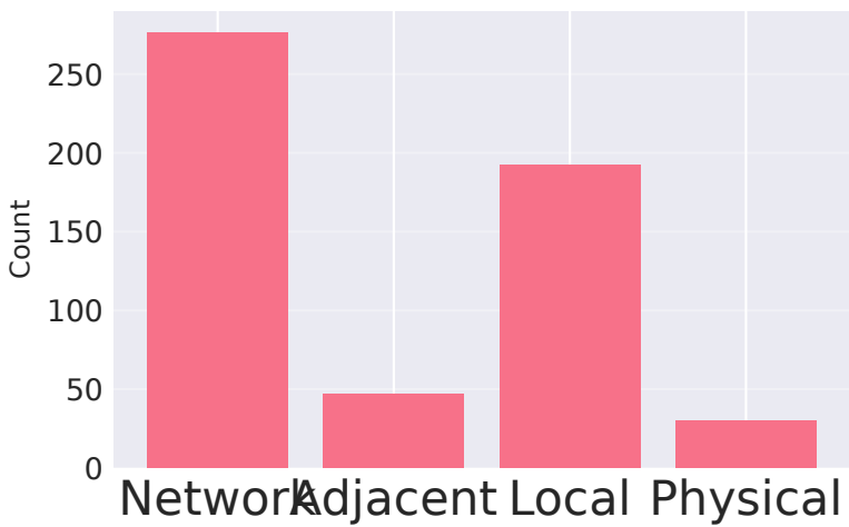
Attack Vector
