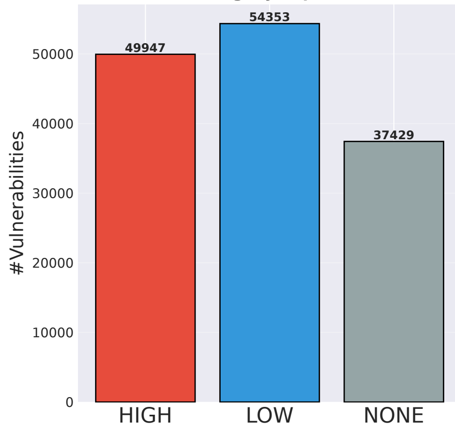
Integrity Impact
