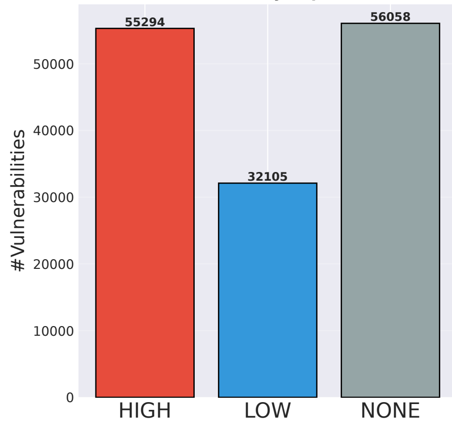
Availability Impact
