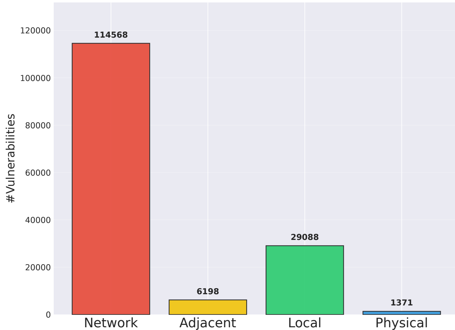
Attack Vector
