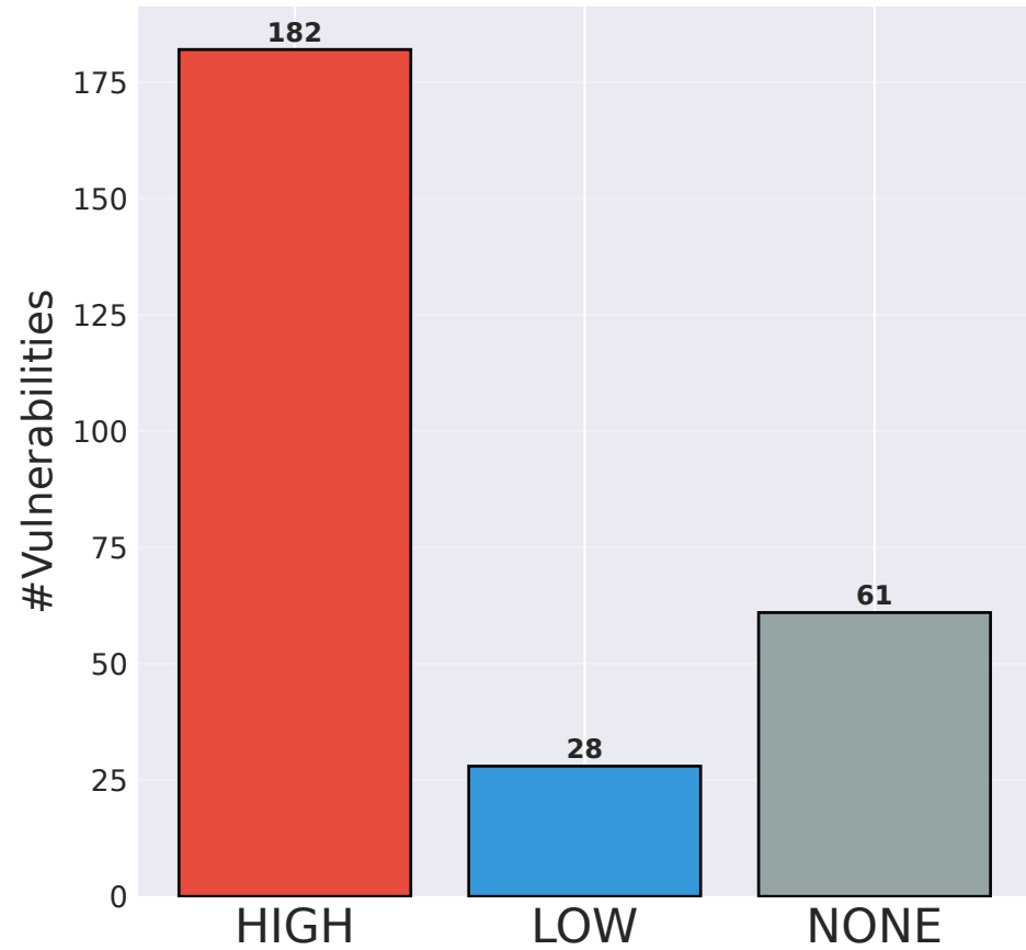
Confidentiality Impact
