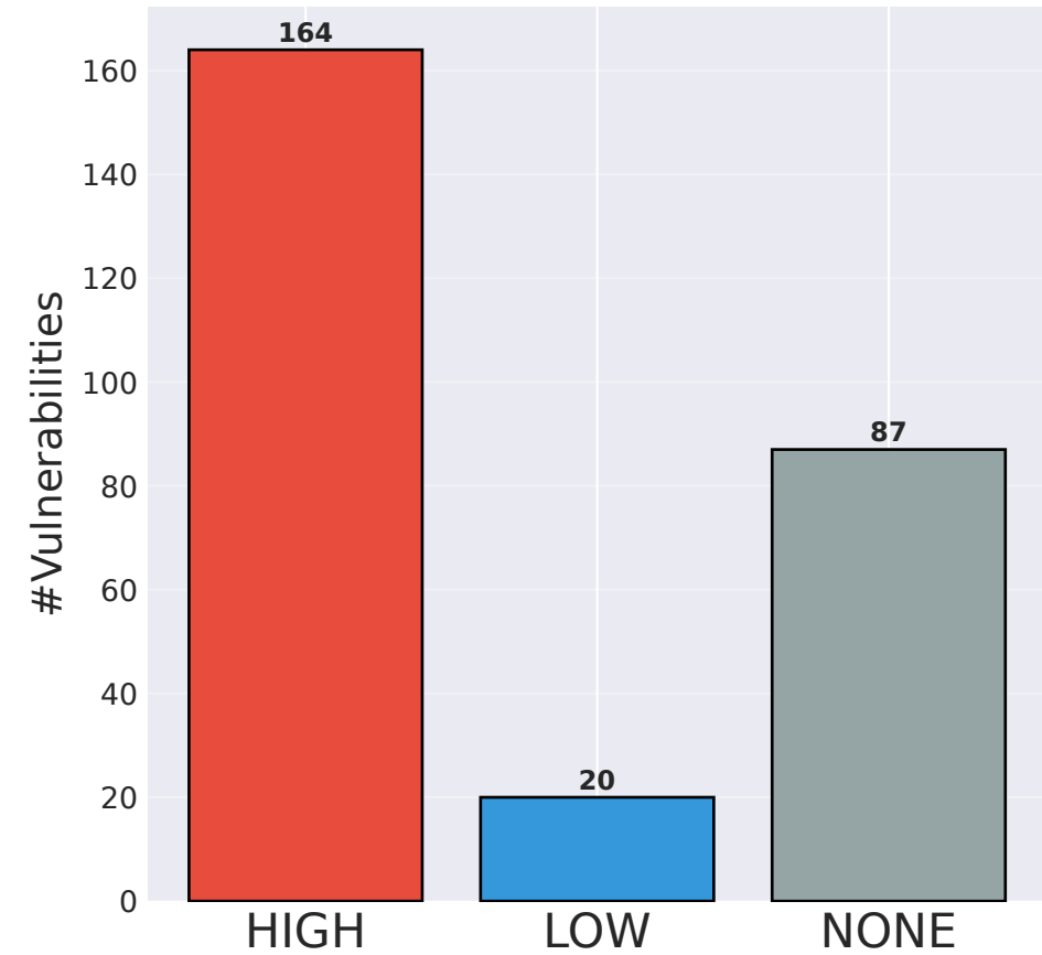
Availability Impact
