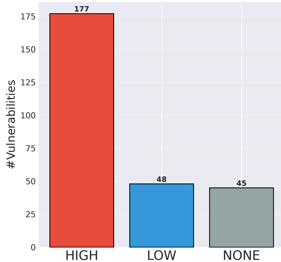
Integrity Impact
