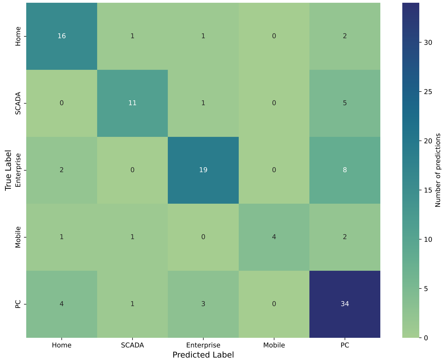
Confusion Matrix - Balanced Linear SVM
