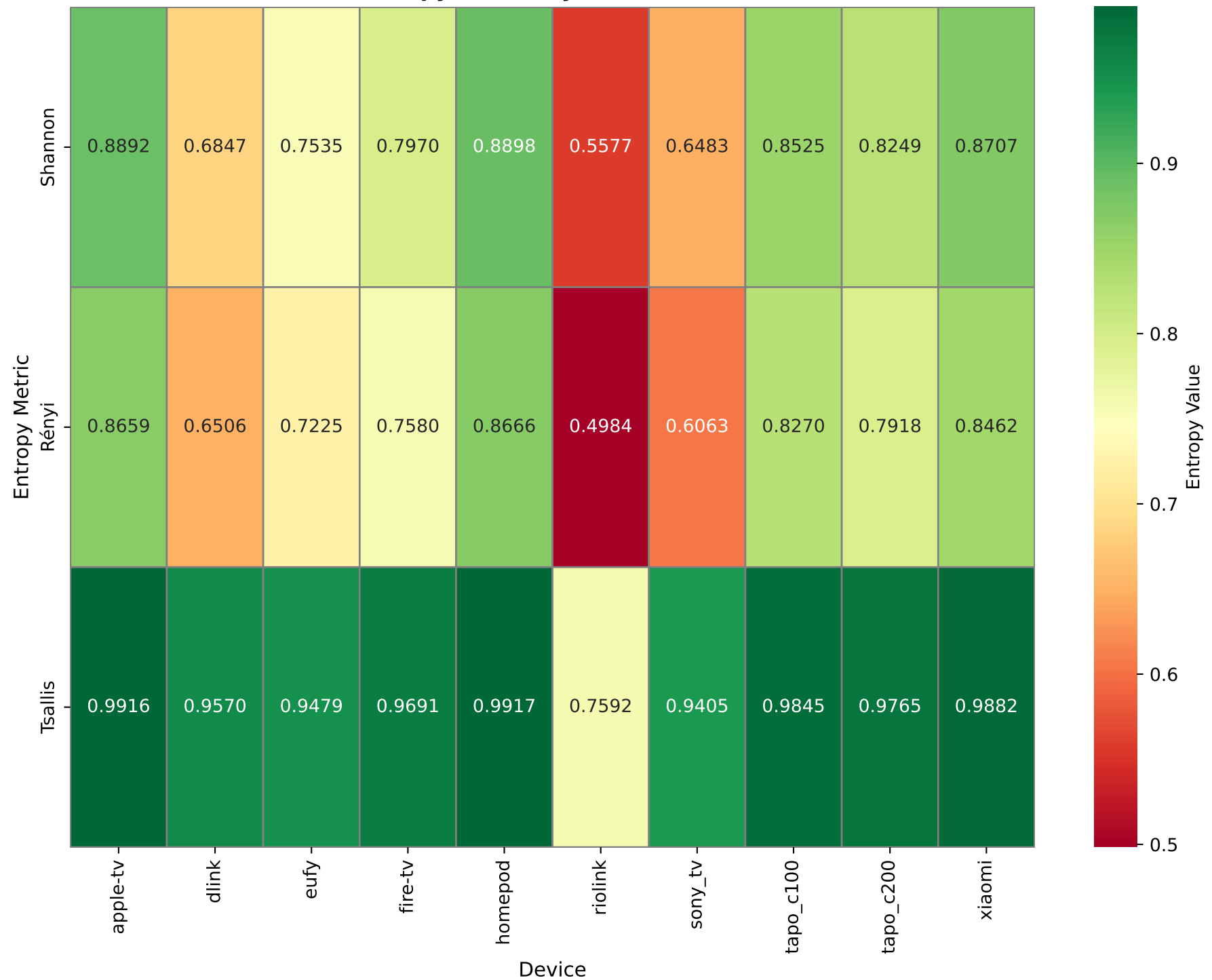
Mean Entropy Values by Device (10 Devices)
