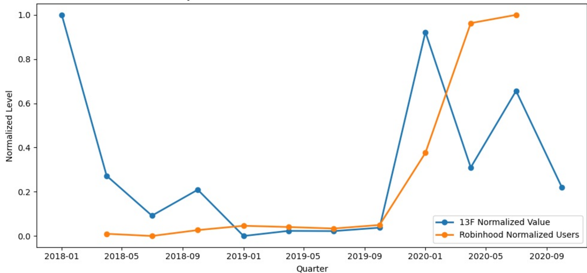
JPM — Normalized 13F Value vs. Robinhood Users
