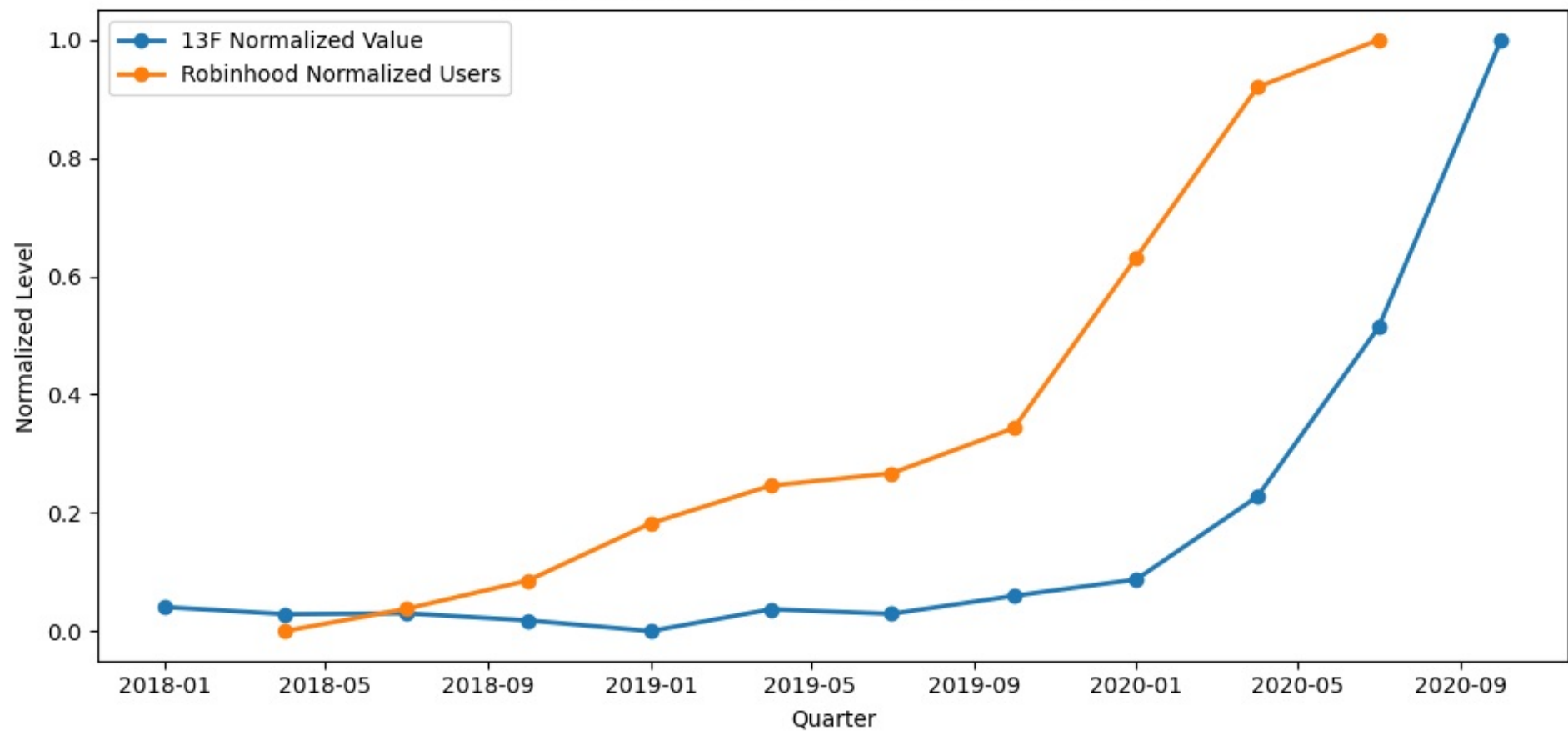
PLUG — Normalized 13F Value vs. Robinhood Users
