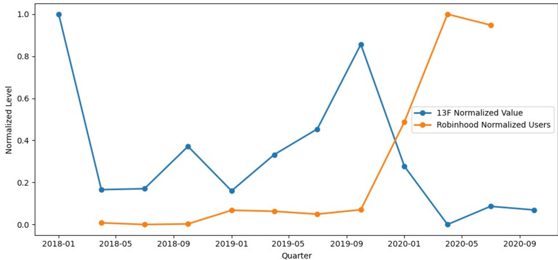
BA — Normalized 13F Value vs. Robinhood Users
