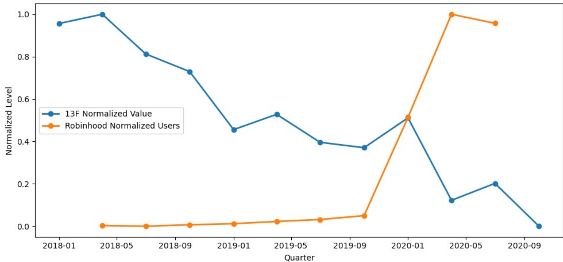
XOM — Normalized 13F Value vs. Robinhood Users
