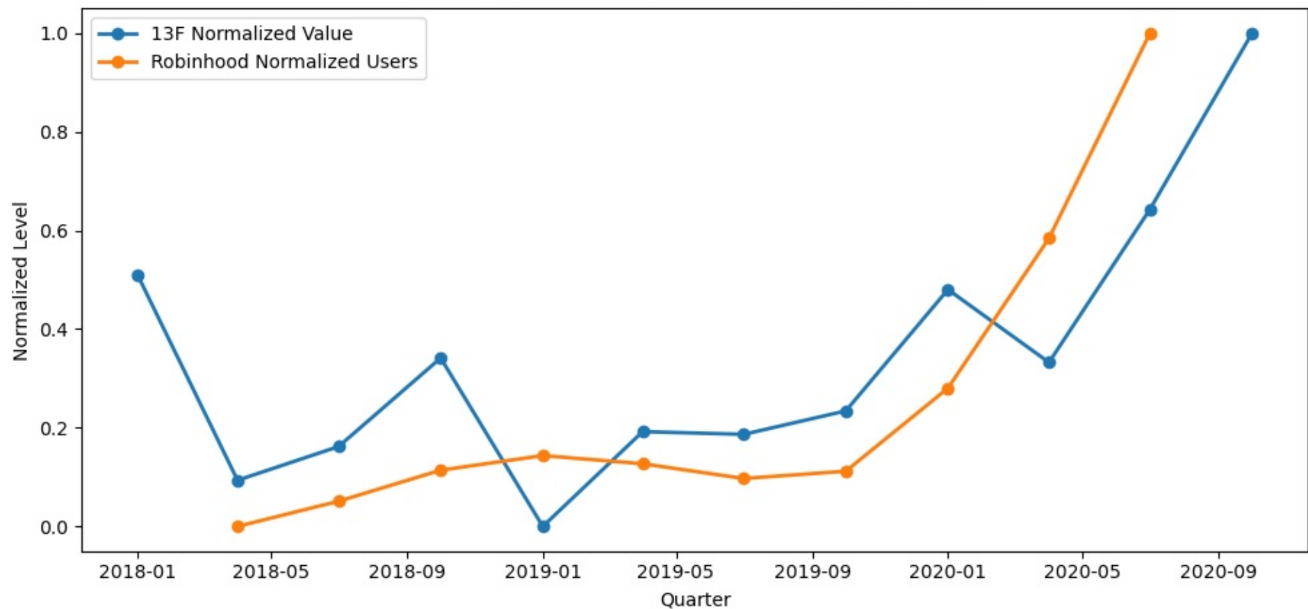
AAPL — Normalized 13F Value vs. Robinhood Users
