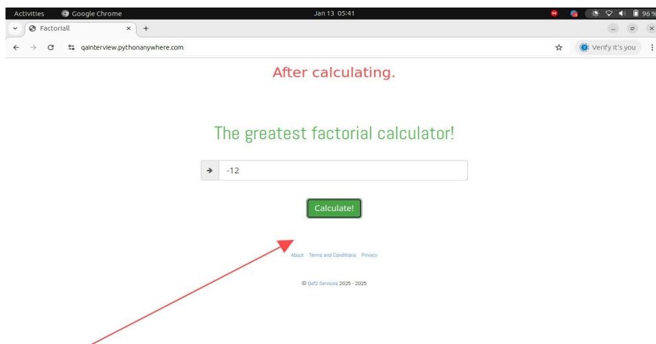
Figure 2: After attempting to calculate the factorial of a negative integer
