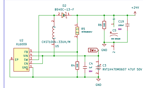
XL6009 Boost-Converter 12 to 24 V
