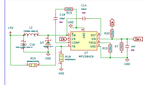
Step Down
