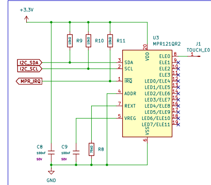
MPR121QR2 I2C
