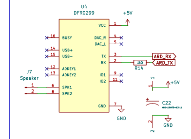
DFR0299 &amp; Speaker
