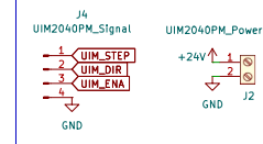
UIM2040PM
