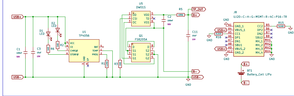
TP4056 Charger Circuit
