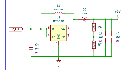
MT3608 DC-DC Step Up
