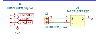
UIM2040PM
