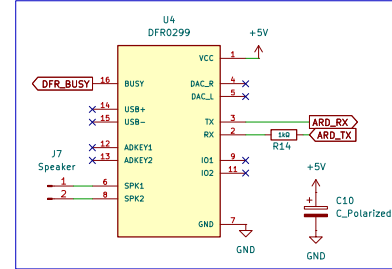
DFR0299 & Speaker
