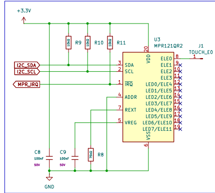
MPR121QR2 I2C
