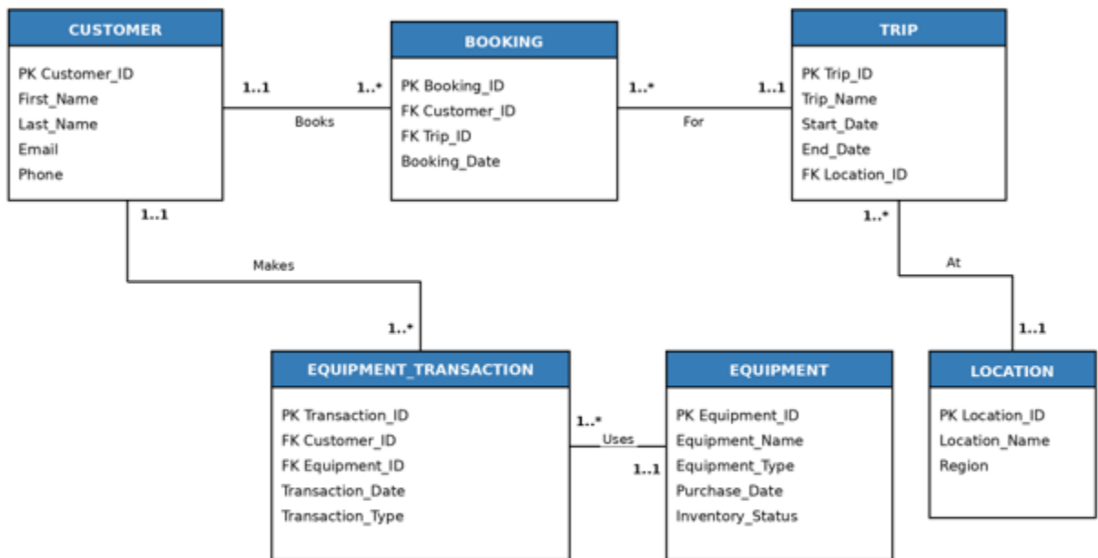
Figure 1. Revised Entity Relationship Diagram for Outland Adventures
