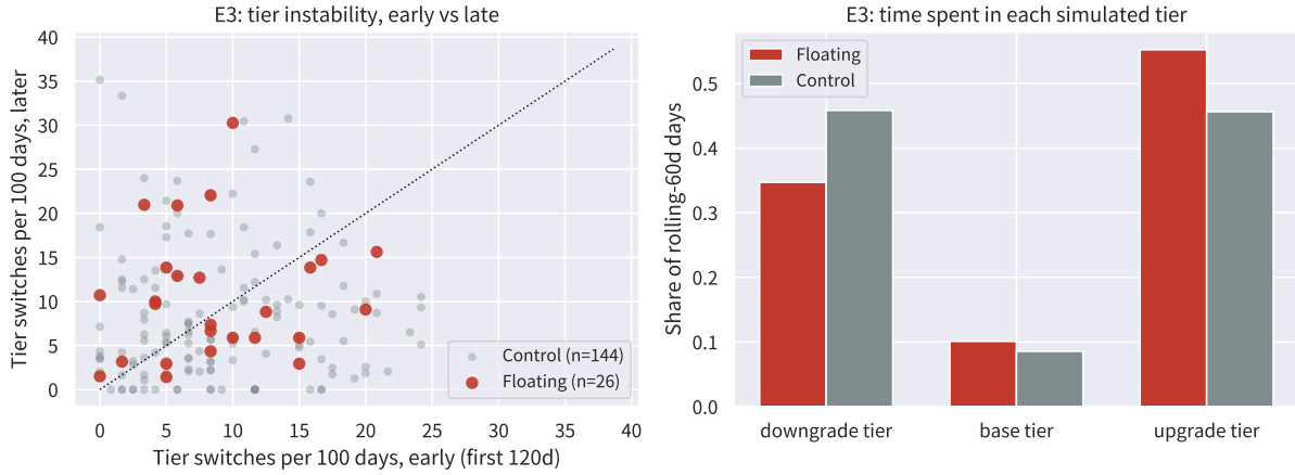
Figure 8: Simulated tier dynamics on rolling 60-trading-day windows: switches per 100 trading days (overall and early vs. late) and dwell shares by tier, floating versus control. The base tier is nearly uninhabited in both groups.
