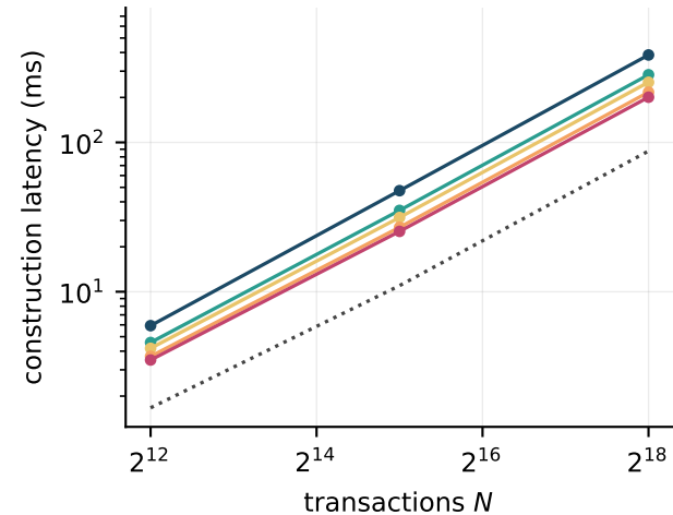
SHA-256
