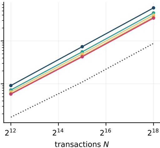
SHA3-256
