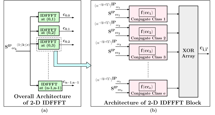
Fig. 14. (a) Hardware architecture of the 2-D IDFFFT unit. It consists of n^2 parallel IDFFFT units that produce the IDFFFT at each point in the n \times n array. (b) Each IDFFFT unit consists of parallel conjugate class units to evaluate the IDFFFT at a certain point.
