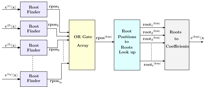
Fig. 11. Architecture of the common connection polynomial finder. Root finders find root positions of the connection polynomials, followed by an OR array which finds positions of common roots. The roots are then converted to the coefficients of the common connection polynomial.
