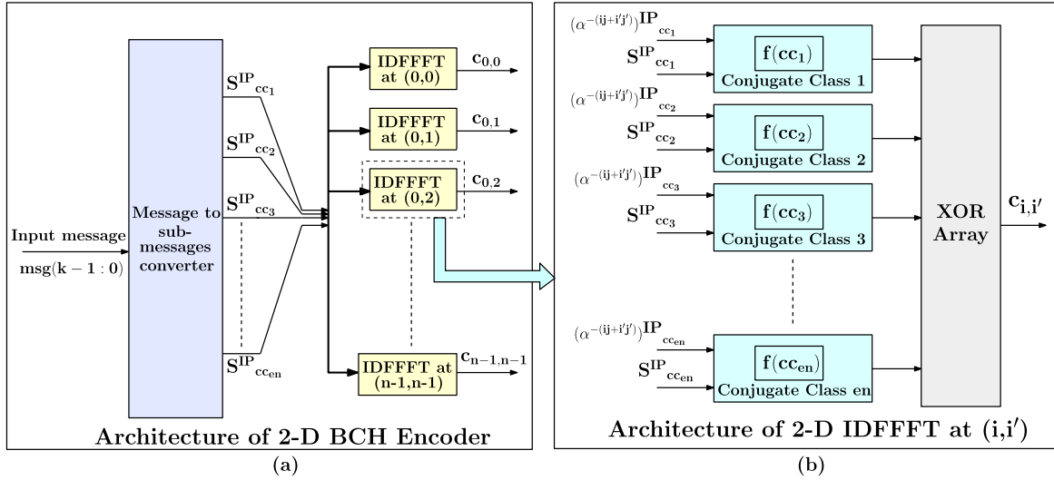
Fig. 5. (a) Overall architecture of the encoder contains n^2 units to compute the 2-D IDFFFT at all (i, i') . (b) Architecture of the IDFFFT block consists of cc_{en} parallel units to compute the 2-D IDFFFT at a certain point (i, i') . Conjugate class unit uses the reduced architecture, as explained in Section III-B.
