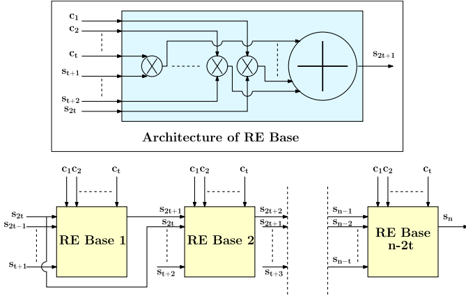
Fig. 13. Hardware architecture of the RE unit. RE base consists of GF multipliers and a XOR array, which produces the next syndrome S_{2t+1} . Cascaded stages of the RE base unit can be used to produce the syndromes of the entire row/column in a single clock cycle.
