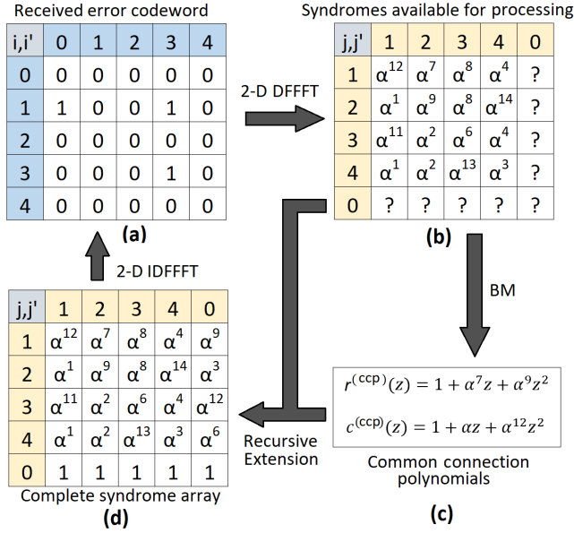
Fig. 6. Decoding example using a BCH code of size 5 \times 5 with t = 2 . (a) Received error codeword. (b) Syndromes available for processing. “?” represents the unknown positions in the spectral domain. (c) Common connection polynomials for row and column. (d) Complete syndrome array produced by RE.
