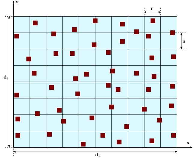
Fig. 1. Tiling of an n \times n 2-D BCH code with a burst error correction capability t \times t . The n \times n squares represent the individual 2-D BCH encoded arrays and the small maroon squares represent a burst of size t \times t .
