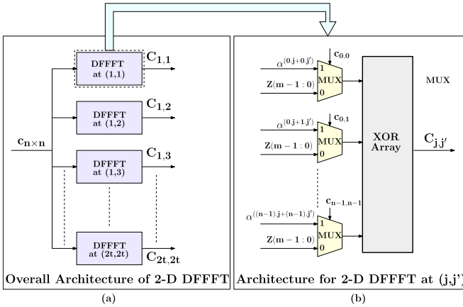
Fig. 9. (a) Hardware architecture of the 2-D DFFFT unit. It consists of 2t \times 2t parallel DFFFT units that compute the 2-D DFFFT at (j, j') for 1 \leq j, j' \leq 2t . (b) Each DFFFT unit consists of n^2 parallel multiplexers that calculate the DFFFT at a certain point using MUX-es and a XOR array.
