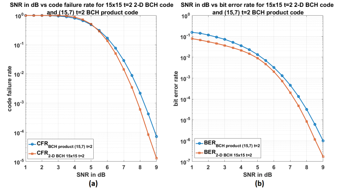
Fig. 7. (a) SNR in dB versus CFR for 15 \times 15 , t = 2 2-D BCH codes and (15, 7) BCH product code with t = 2 . (b) SNR in dB versus BER for 15 \times 15 , t = 2 2-D BCH codes, and (15, 7) BCH product code with t = 2 .
