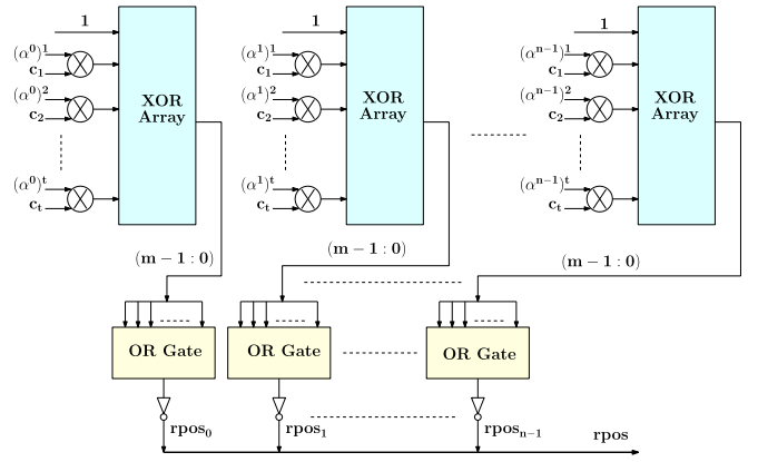
Fig. 12. Architecture of the root finder unit. n parallel stages test whether each element in \text{GF}(2^m) is a root of the connection polynomial.
