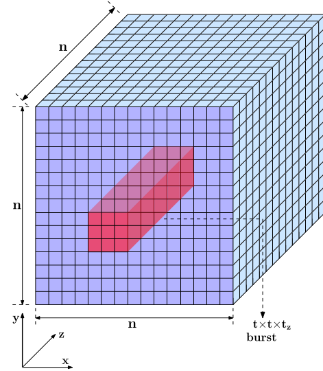
Fig. 2. Tiling of n 2-D BCH codes of dimensions n \times n in 3-D space for correction of burst errors along the z -axis. A t \times t \times t_z burst is shown in red.
