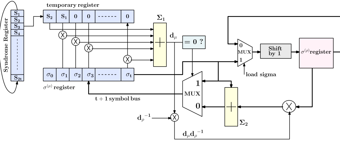
Fig. 10. Architecture of BM engine. The main steps in this stage are to find the discrepancy factor ( d_\mu ) and the correction factor d_\mu d_\rho^{-1} x^{(\mu-\rho)} \sigma^{(\rho)}(x) , which will be used to update \sigma^{(\mu+1)}(x) for the next iteration [1].
