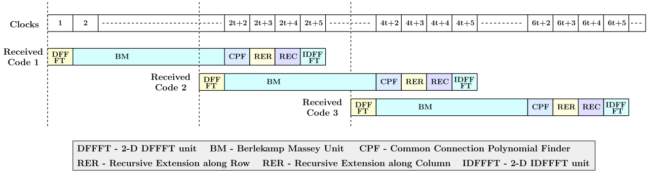
Fig. 15. Decoder consists of six pipelined stages, namely the 2-D DFFFT unit, the BM engine, the common connection polynomial finder, RE unit along row, RE unit along column, and the 2-D IDFFFT unit. They consume 1, 2t , 1, 1, 1, and 1 clock cycles, respectively. The pipelined architecture has a latency of 2t + 5 clock cycles and produces an output every 2t clock cycles after the first codeword is processed.
