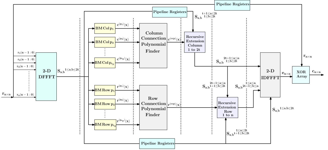
Fig. 8. Top-level architecture of the BCH decoder. It consists of six pipelined stages, namely the 2-D DFFFT, BM engine, connection polynomial finder, RE along rows, RE along columns, and the 2-D IDFFFT unit. The stages take 1, 2t, 1, 1, 1 , and 1 clock cycles. The decoder is a pipelined architecture with a latency of 2t + 5 , able to process a codeword every 2t clock cycles. Each stage is separated using pipeline registers.
