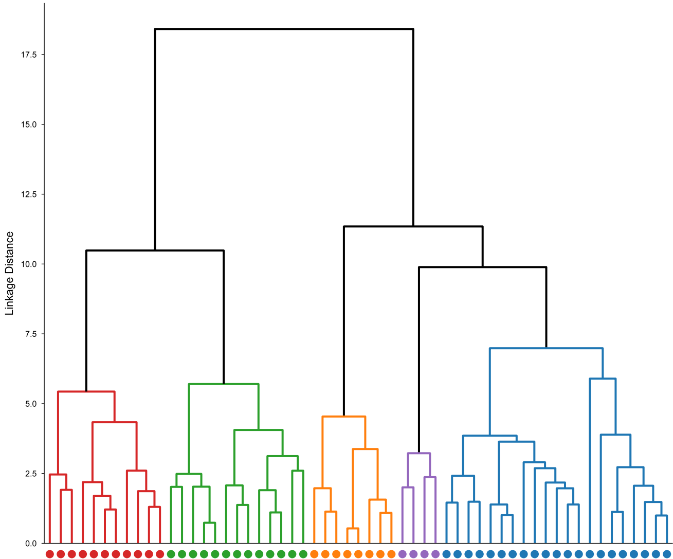
Hierarchical Clustering Dendrogram (pca, 5 clusters, hierarchical)
