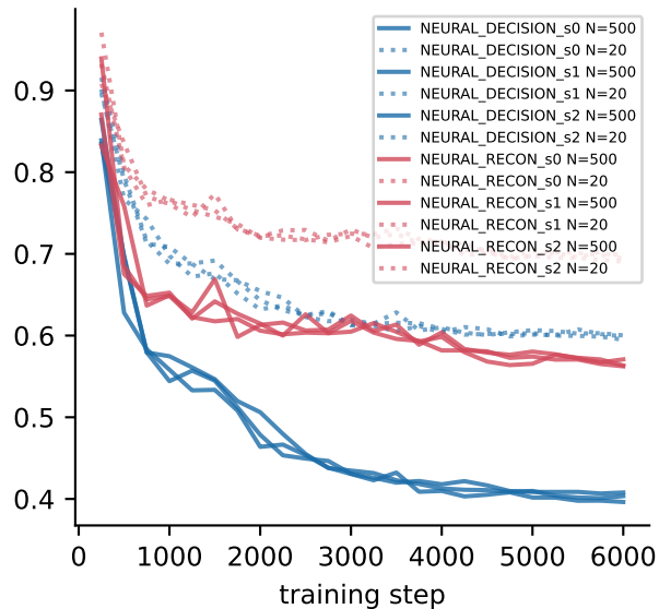
(c) val g-NMSE (solid N=500, dotted N=20)
