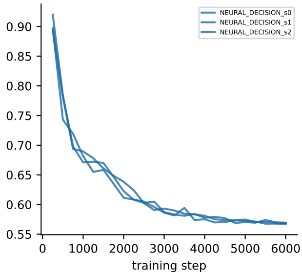
(a) decision: val NMSE(g)
