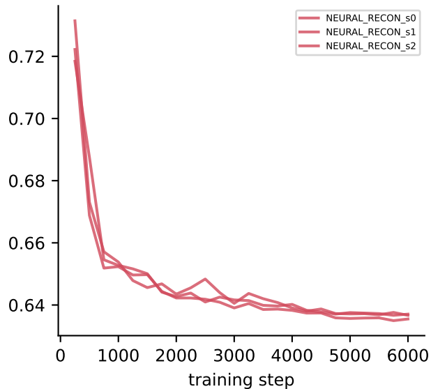
(b) reconstruction: val CE(q)
