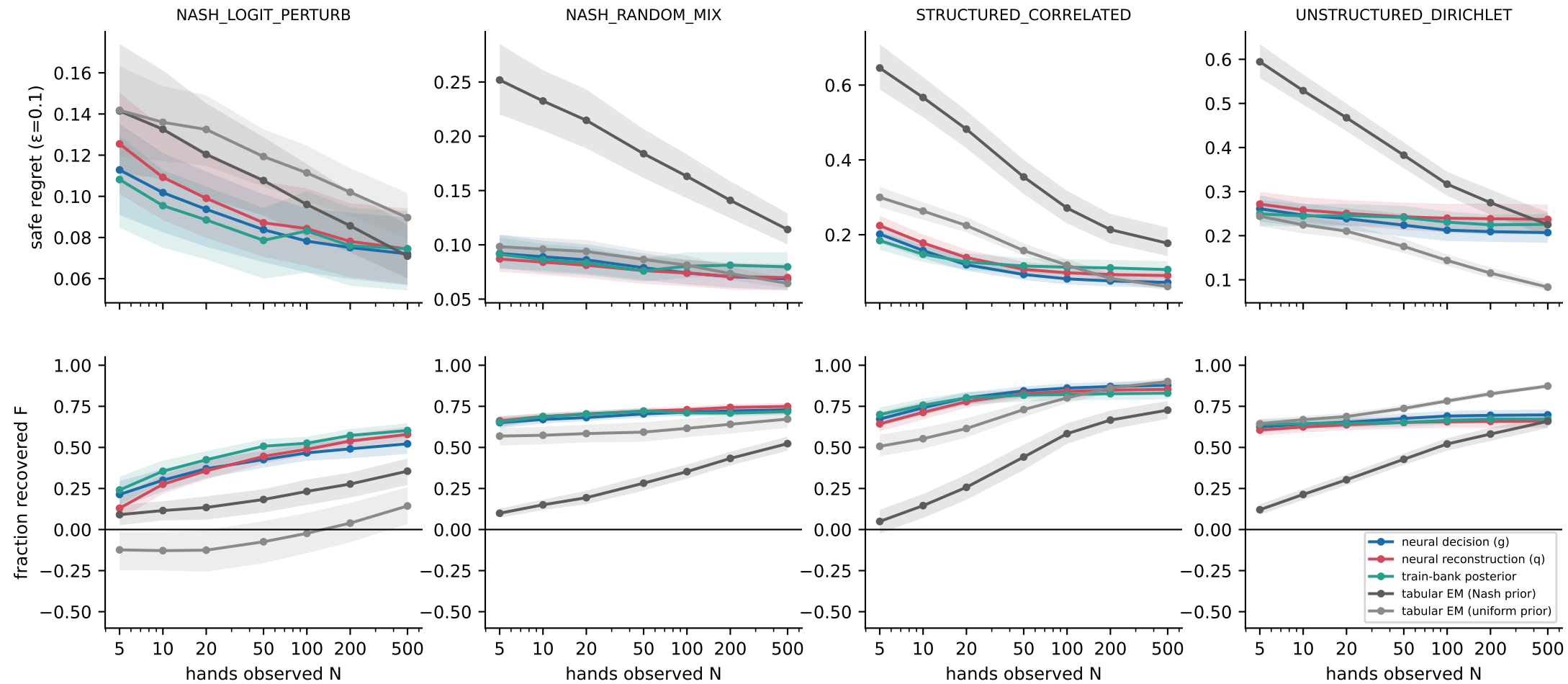
Figure 6: sample efficiency by opponent family ( \varepsilon = 0.1 )
