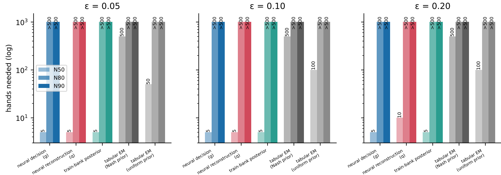
Figure 3: minimum tested N reaching 50 / 80 / 90 % of oracle-safe gain (>500 shown at top)
