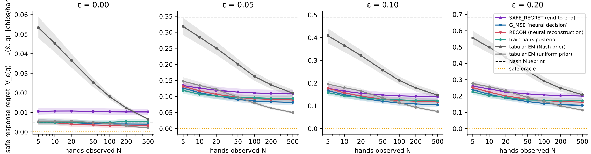
Figure 1: safe response regret vs hands observed (held-out opponents, paired bootstrap 95% CI)
