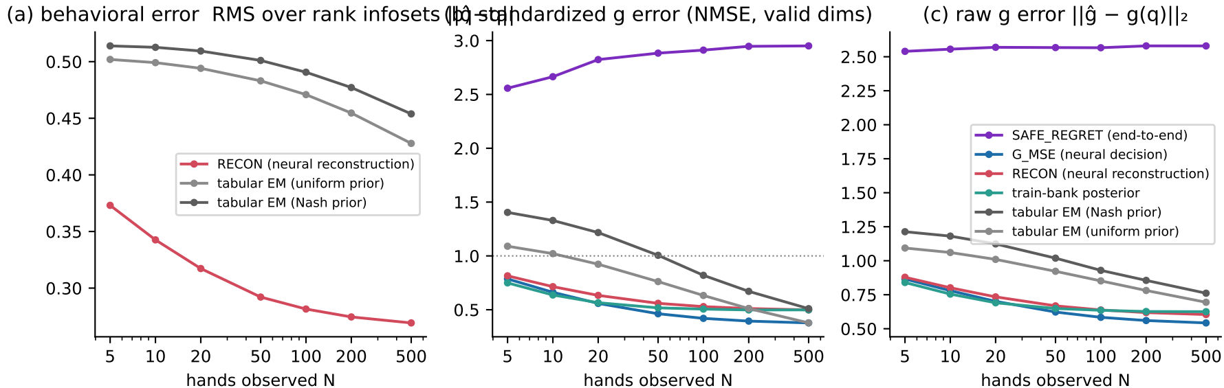
Figure 5: behavioral reconstruction error and decision-vector error vs N (held-out opponents)
